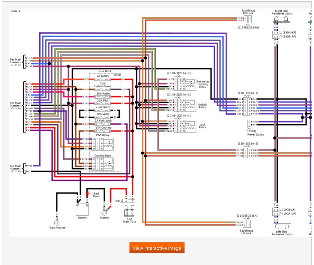
Main Harness (4 of 4): 2019 FLHTKSE
