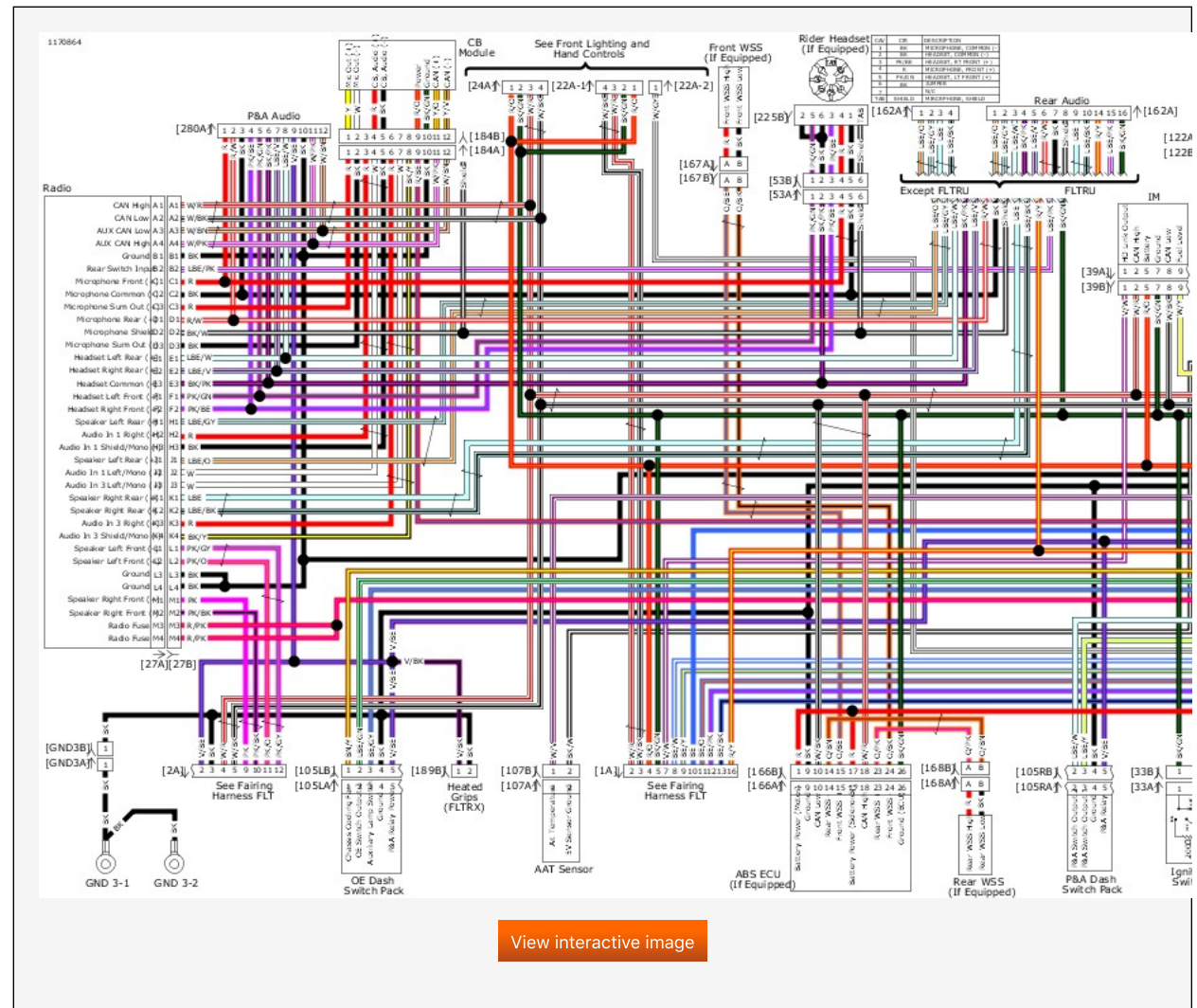
Main Harness FLT 1 of 3: 2019 Touring (with Fairing)
