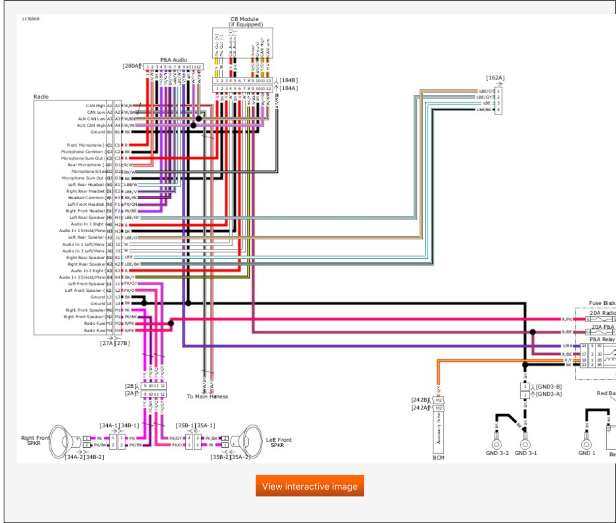
OE Radio: 2019 Touring (No Tour-Pak)
