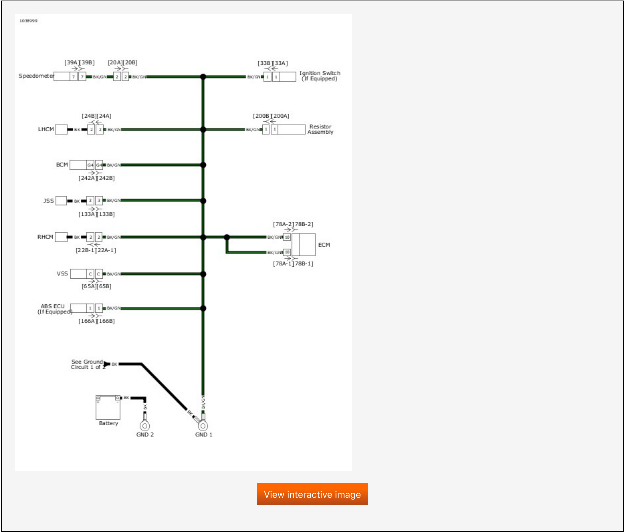
Sensor Grounds
