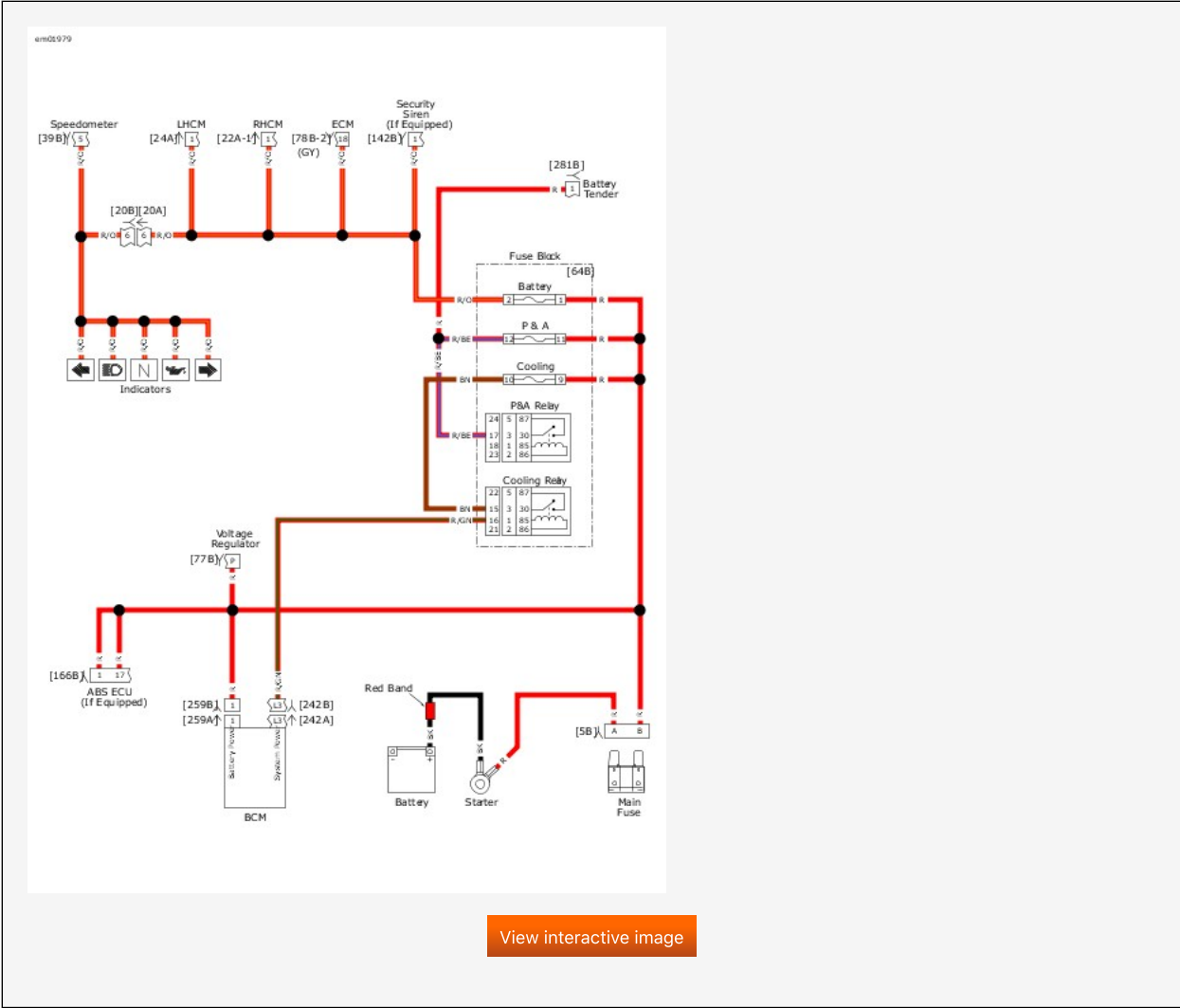
Battery Power Distribution without Fusing
