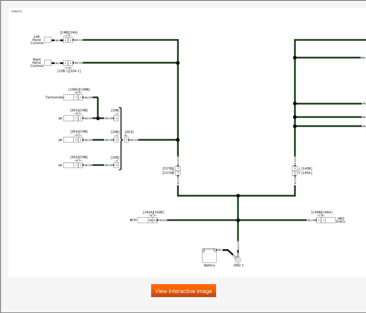
Sensor Grounds: 2019 Softail
