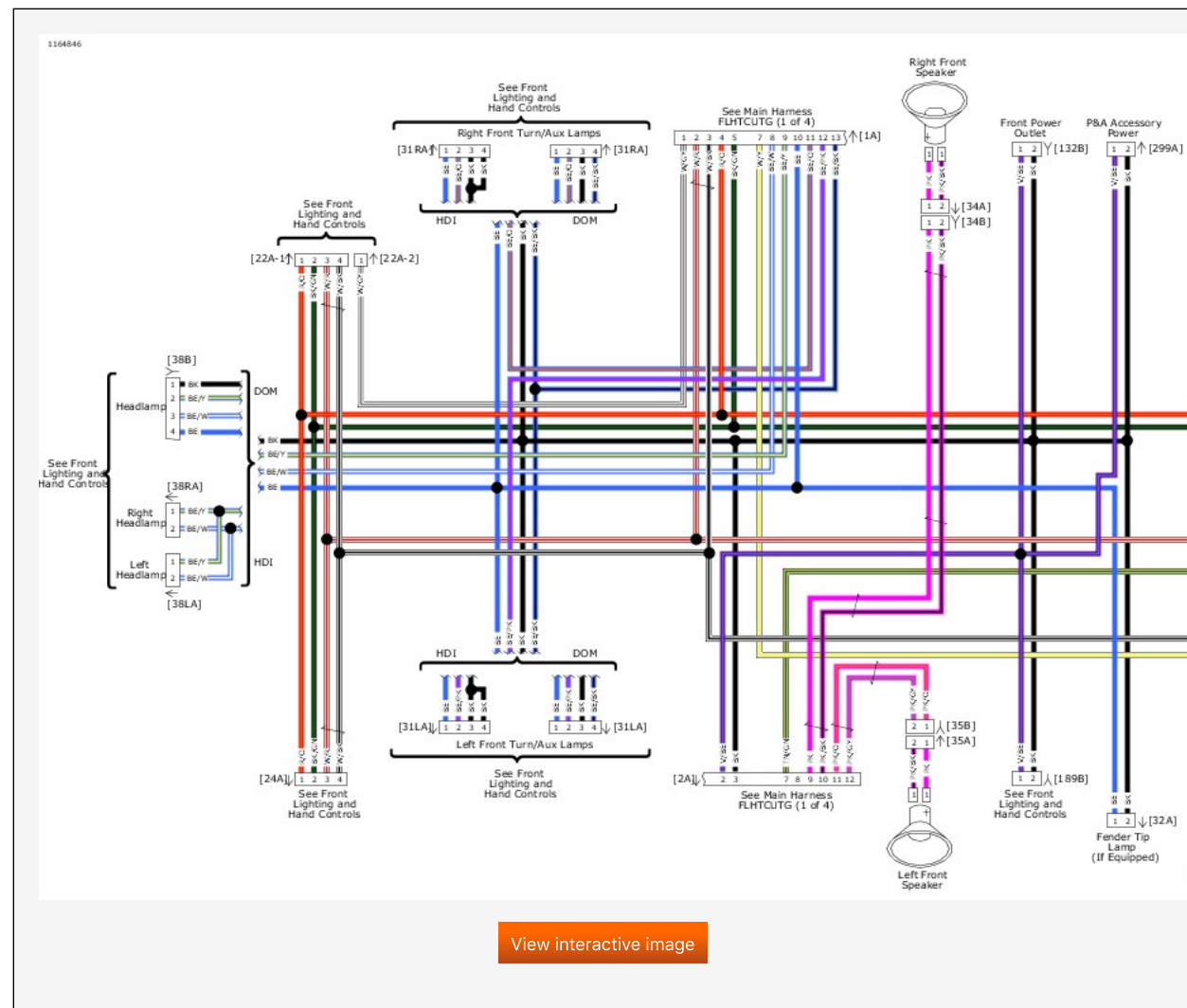
Fairing Harness FLHTCUTG: 2019 Trike Model
