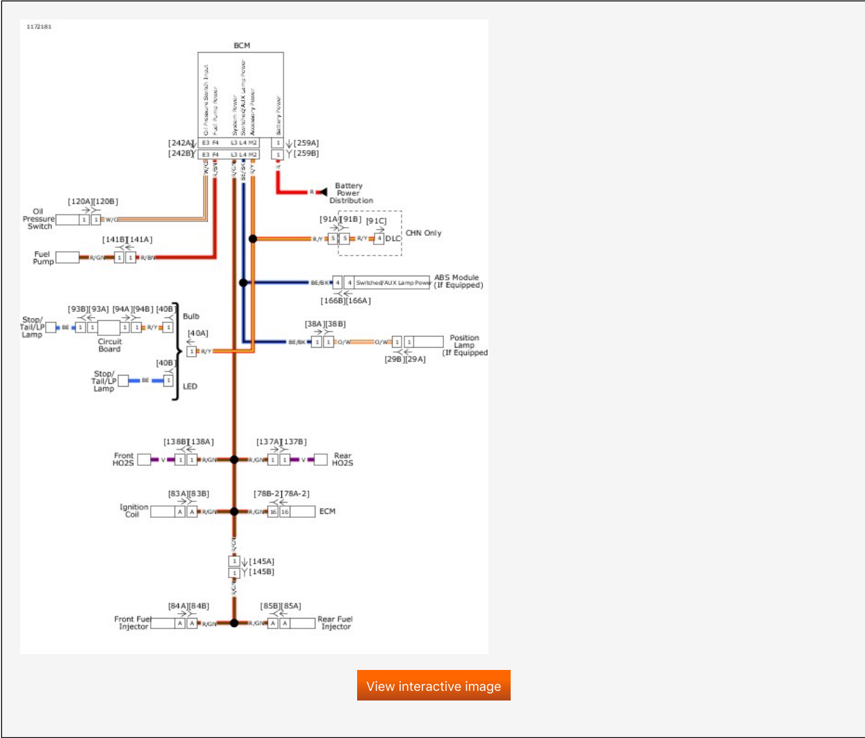
Ignition and Accessory Power Distribution
