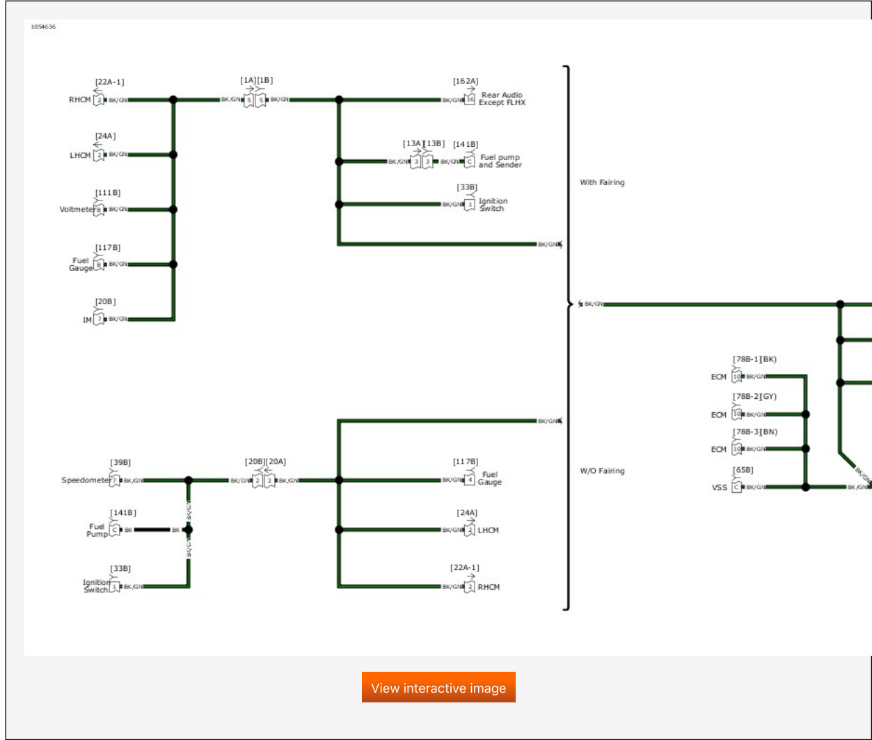
Sensor Grounds FLH: 2019 Touring
