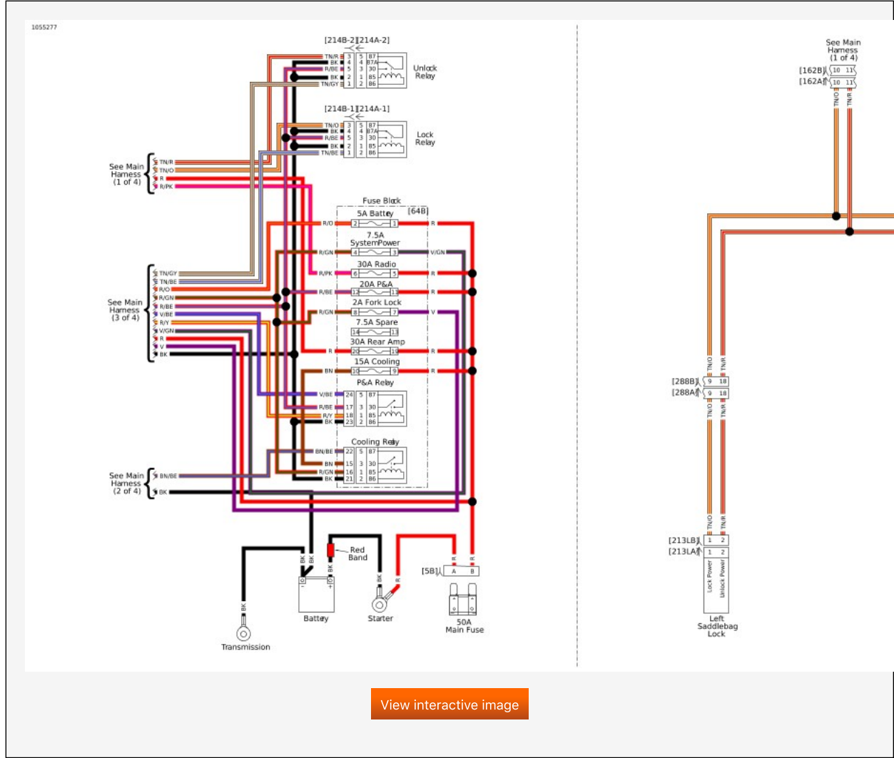
Main Harness (4 of 4): 2019 FLTRXSE
