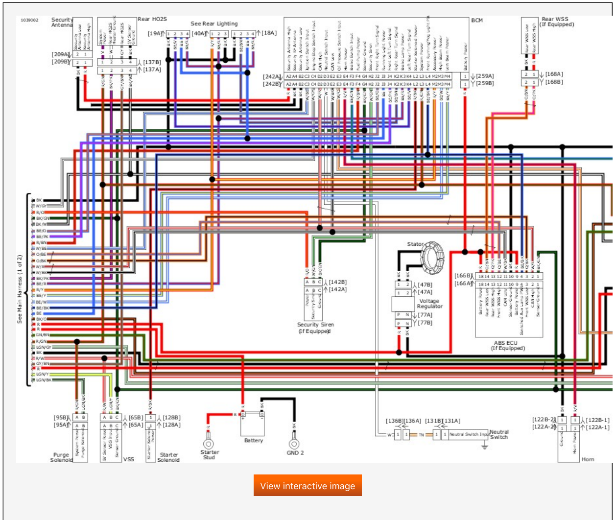
Main Harness 2 of 2: 2019 Sportster
