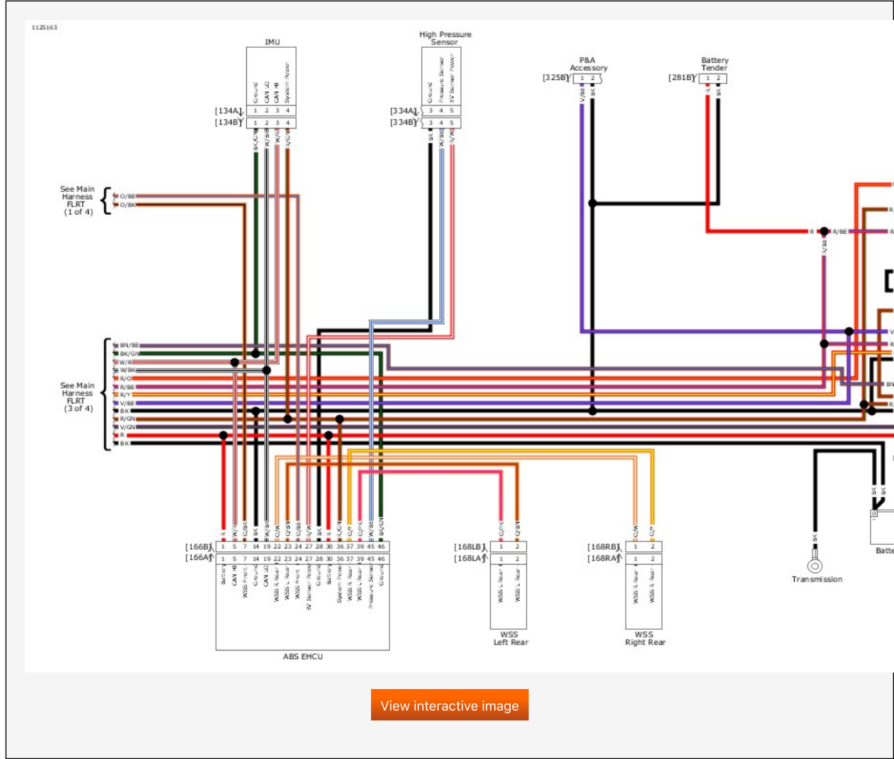
Main Harness FLRT (4 of 4): 2019 Trike Model
