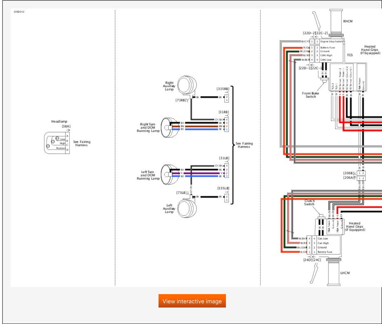
Front Lighting and Hand Controls: 2019 FLHTKSE
