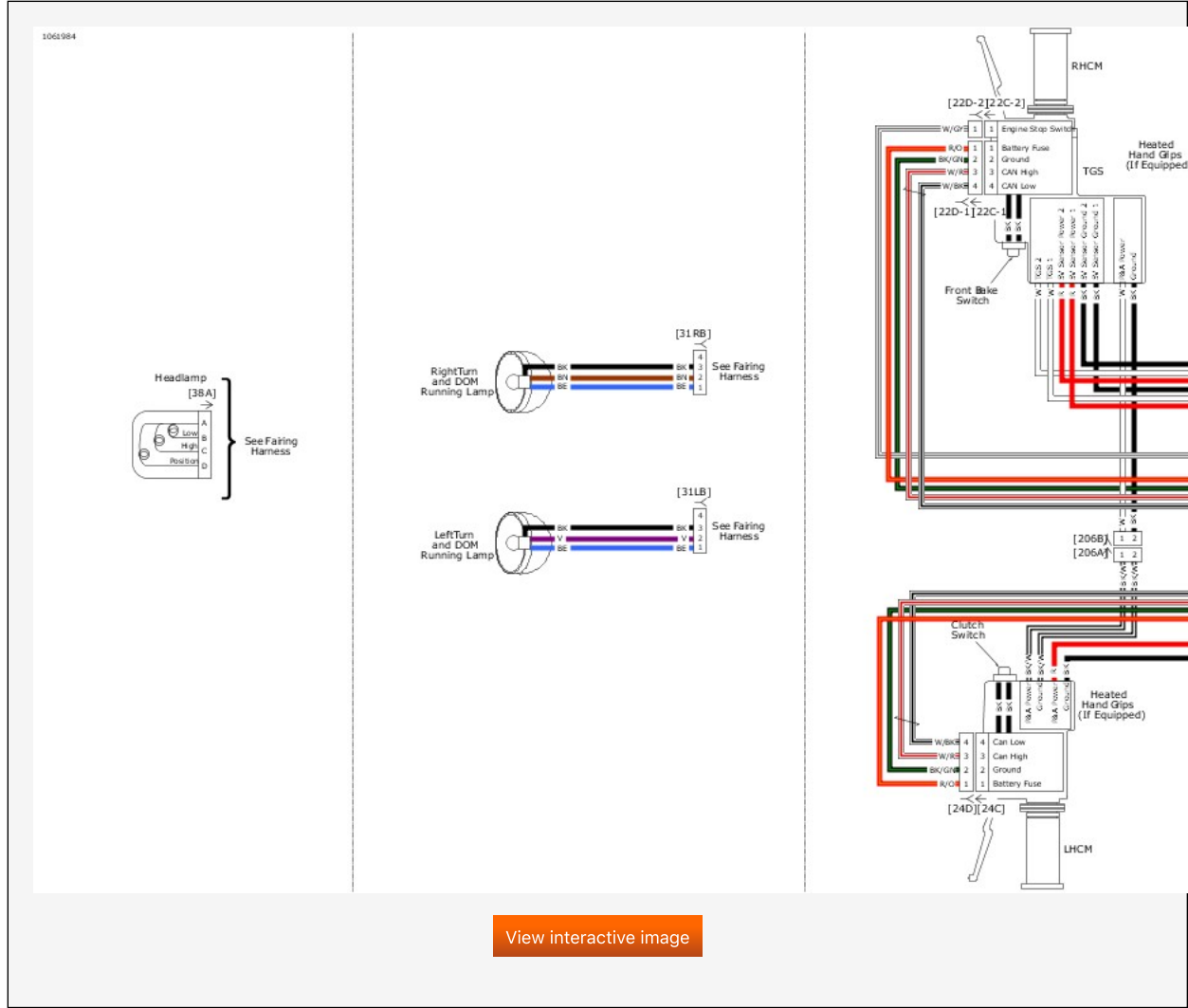
Front Lighting and Hand Controls: 2019 FLTRXSE
