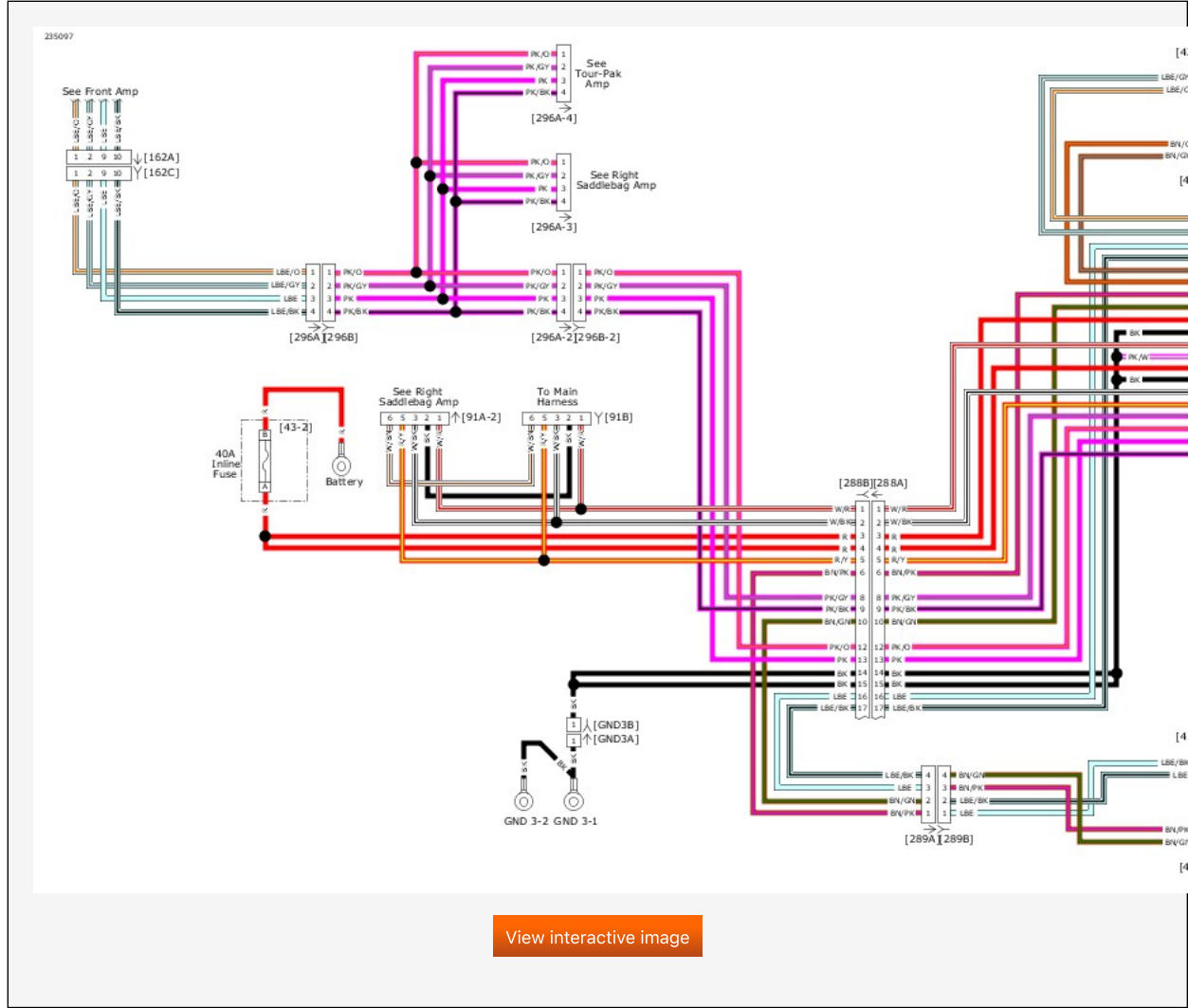
P&A Radio with 4 Amps (2 of 4), Left Saddlebag Amp: 2019 Touring
