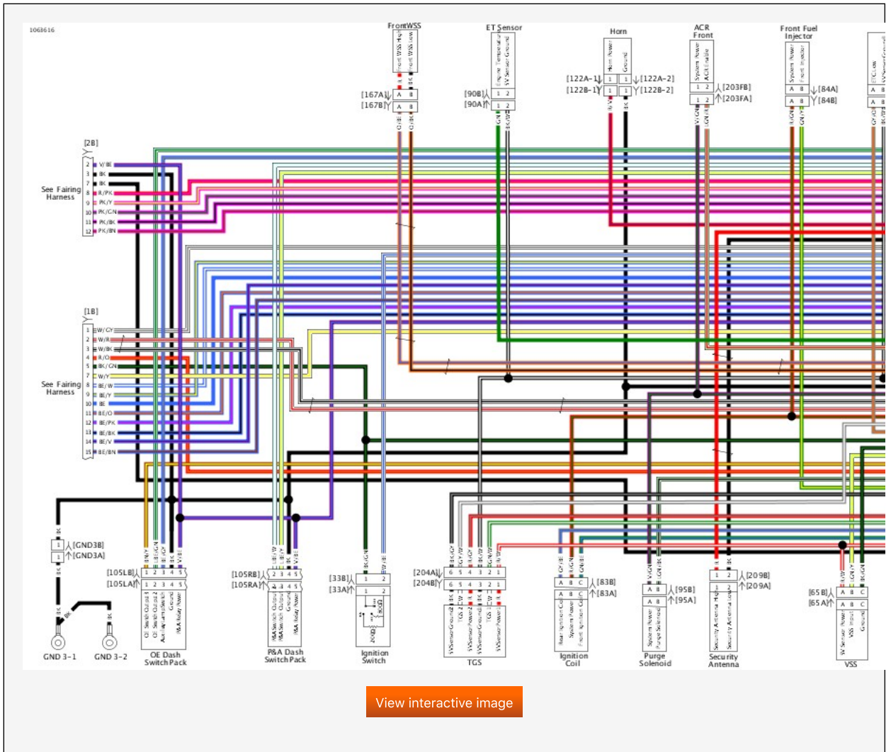
Main Harness (1 of 3): 2019 FLHTP
