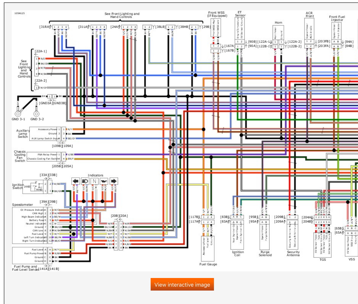
Main Harness (1 of 3): 2019 Touring (without Fairing)
