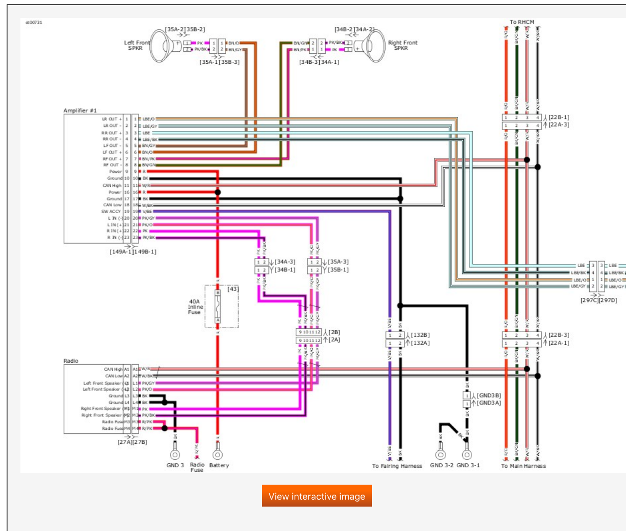
P&A Radio with 2 Amps (1 of 2): 2019 Touring
