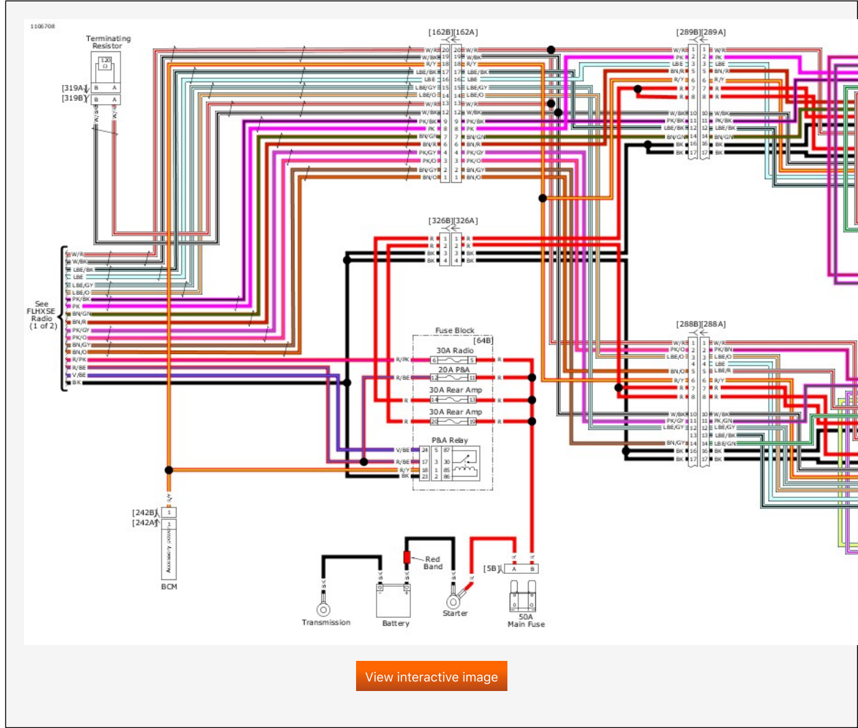
Radio (2 of 2): 2019 FLHXSE
