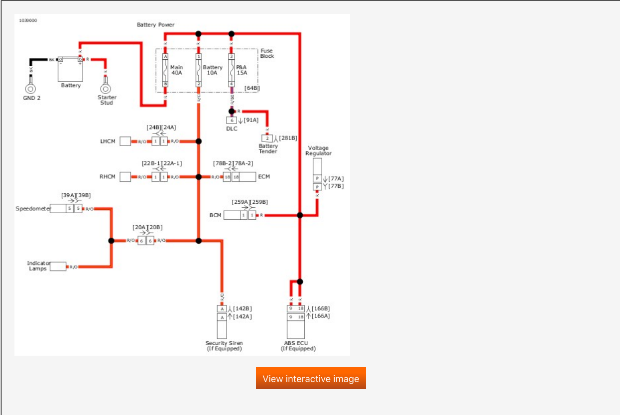
Battery Power Distribution
