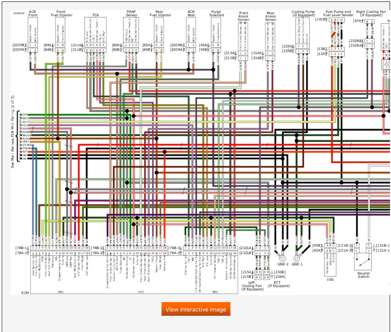
Main Harness FLH (2 of 3): 2019 Touring (with Fairing)
