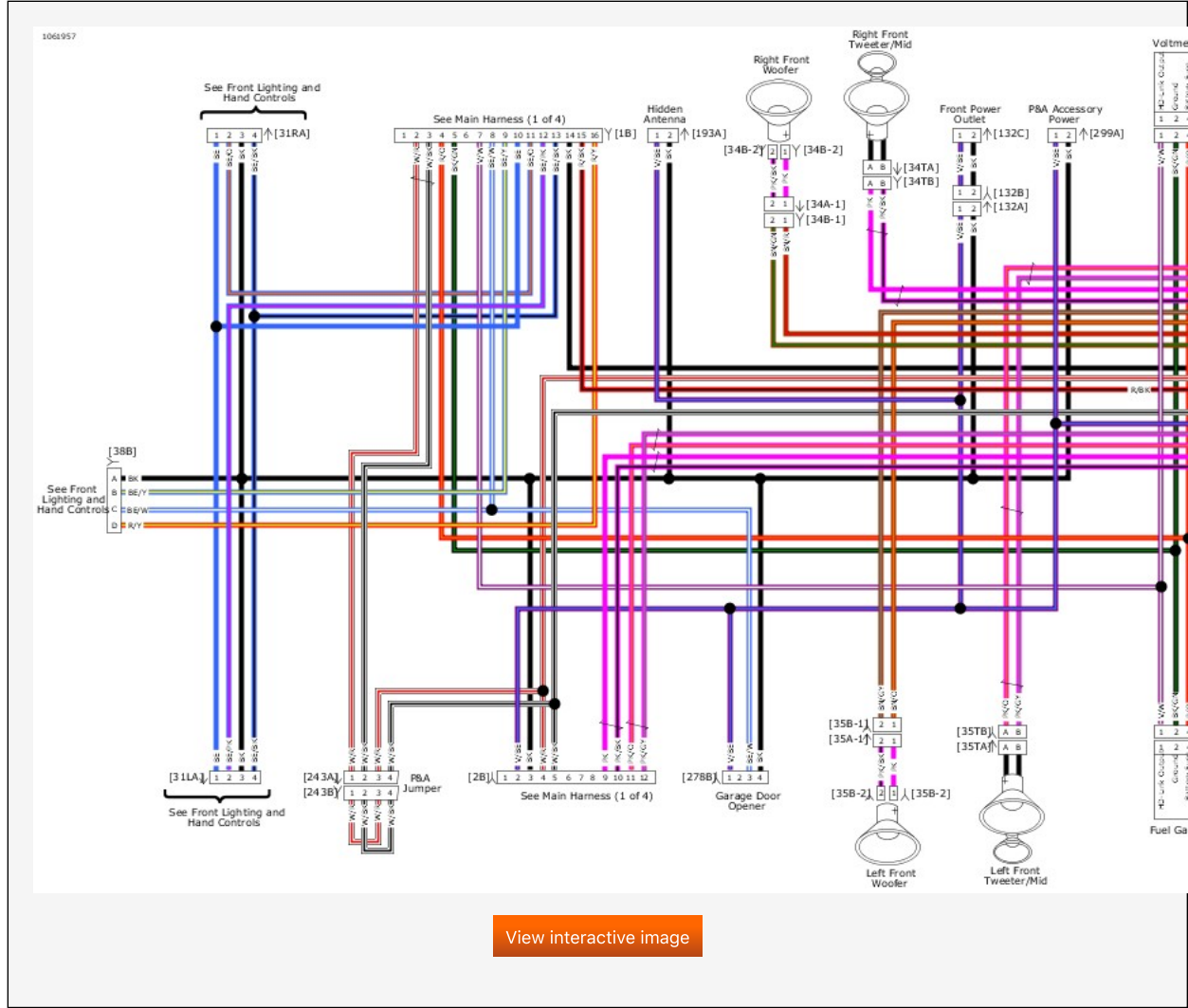
Fairing Harness: 2019 FLTRXSE
