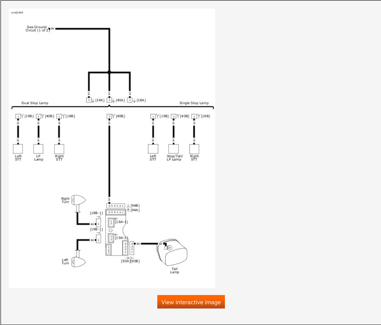
Ground Circuit: 2 of 2
