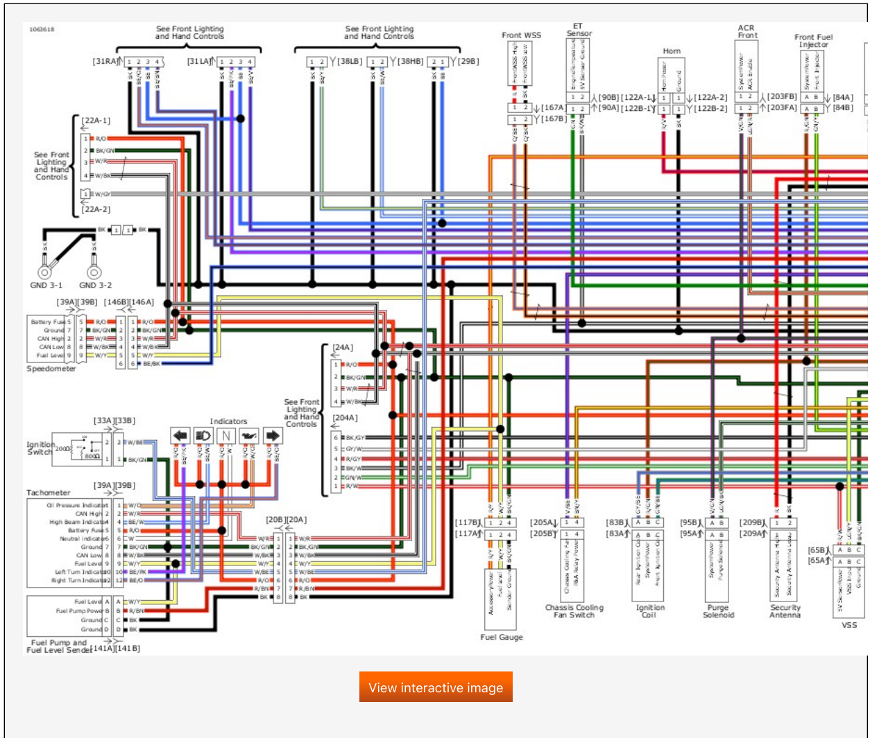
Main Harness (1 of 3): 2019 FLHP
