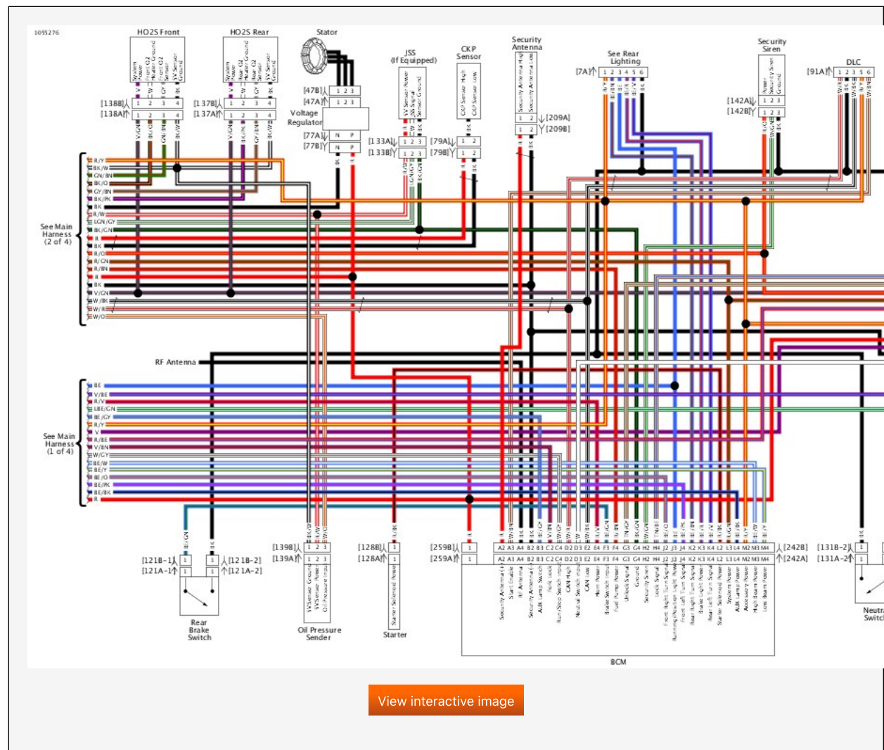
Main Harness (3 of 4): 2019 FLTRXSSE
