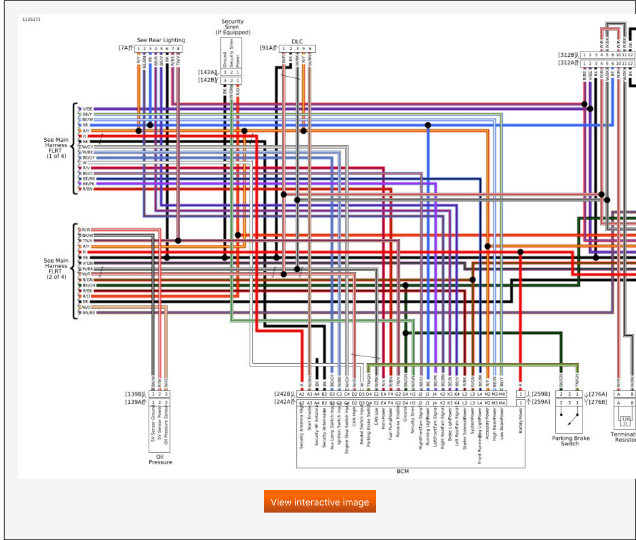
Main Harness FLRT (3 of 4): 2019 Trike Model
