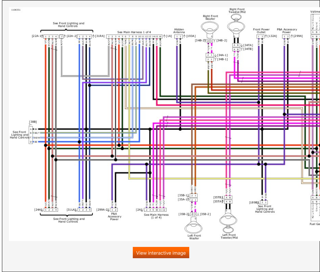
Fairing Harness: 2019 FLHXSE
