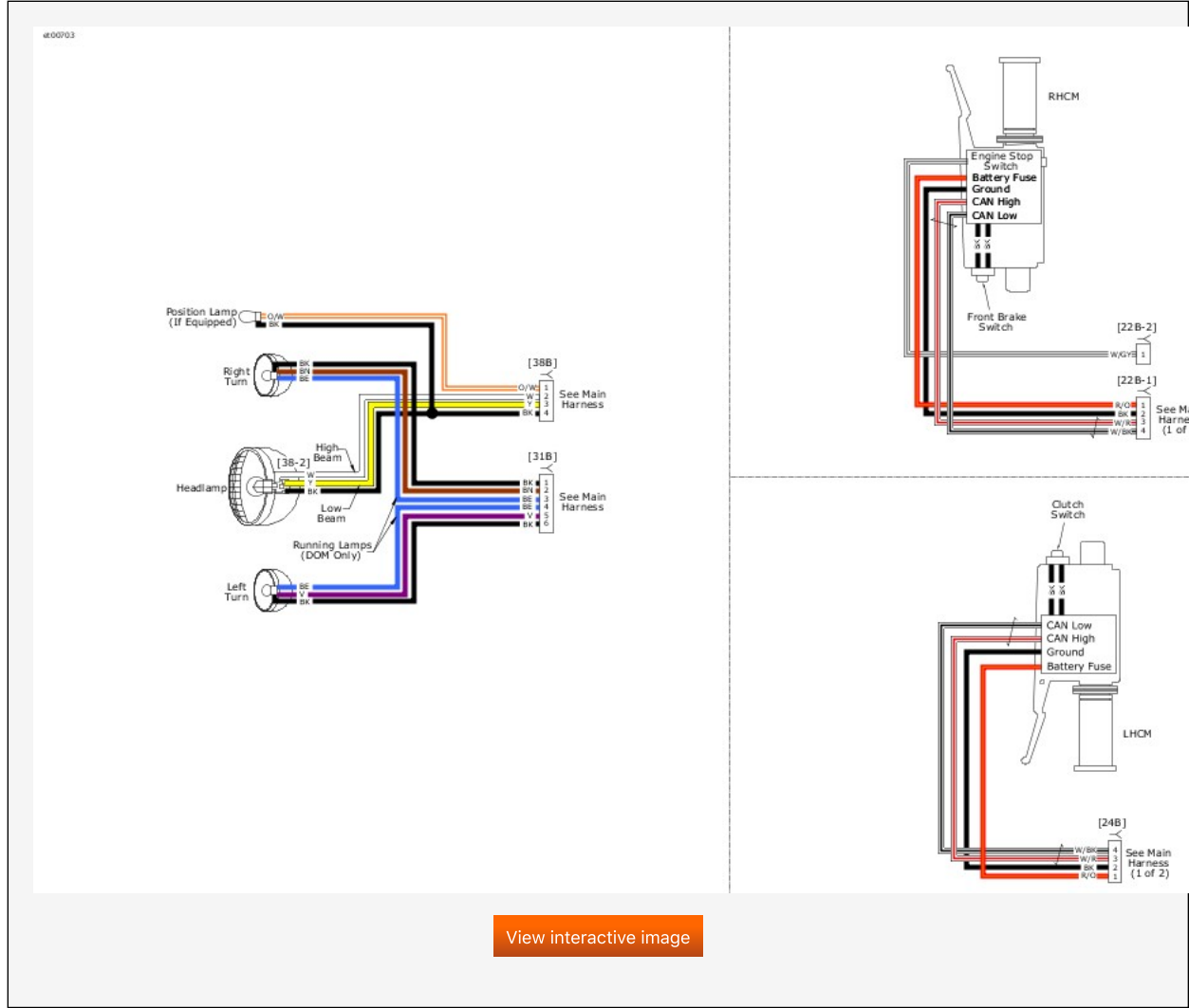
Front Lighting and Hand Controls: 2019 Sportster
