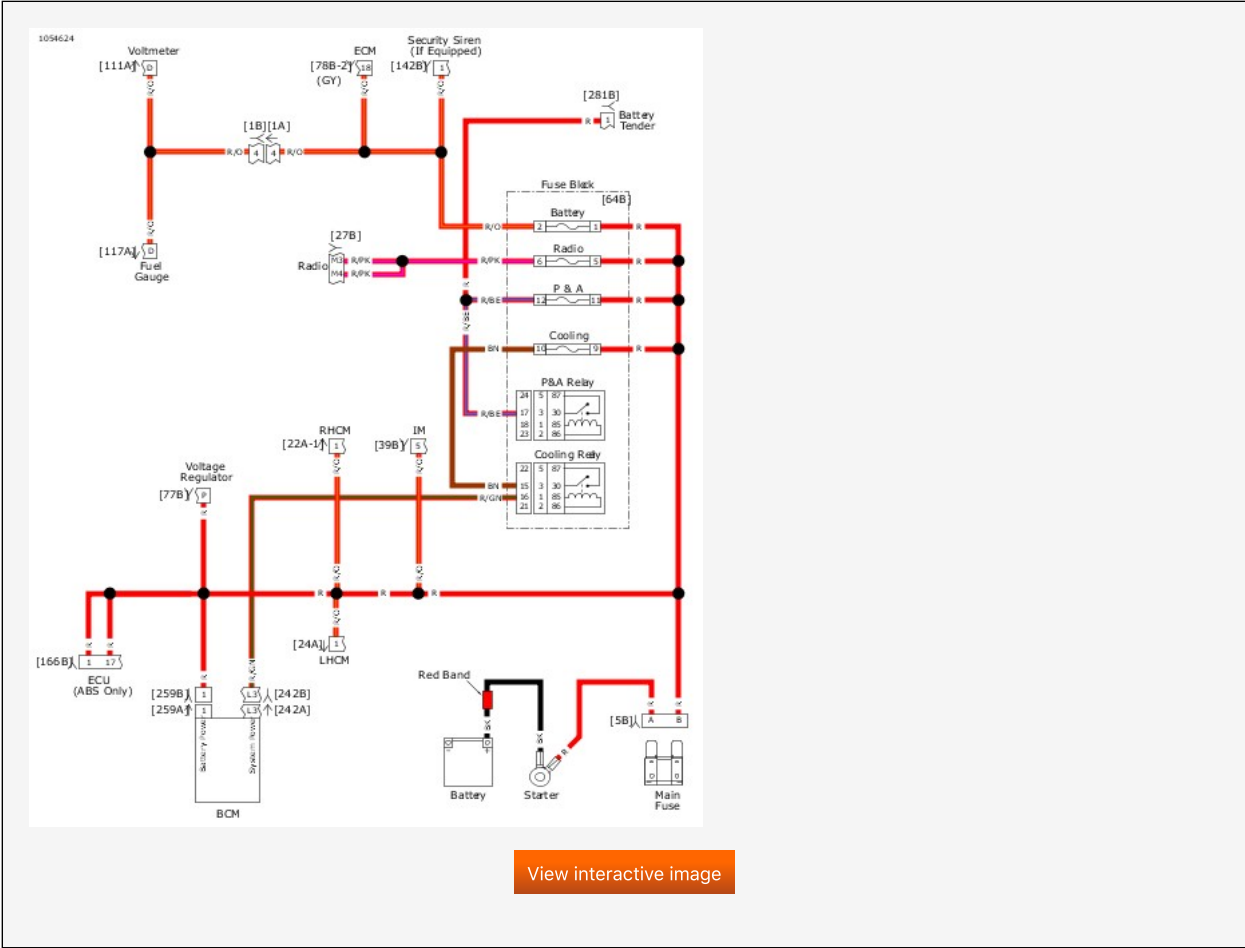
Battery Power Distribution: FLT
