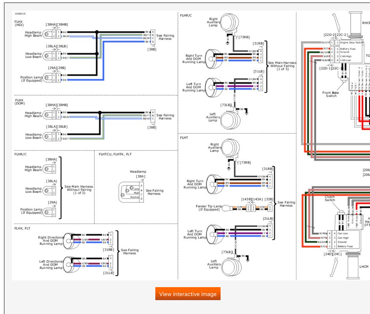
Front Lighting and Hand Controls: 2019 Touring
