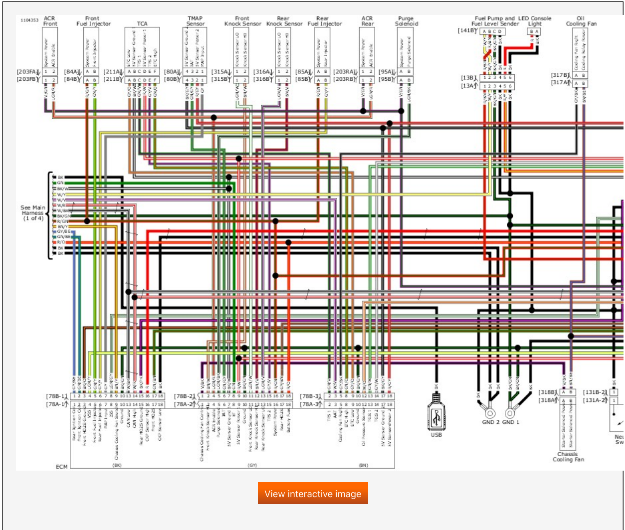
Main Harness (2 of 4); 2019 FLHXSE
