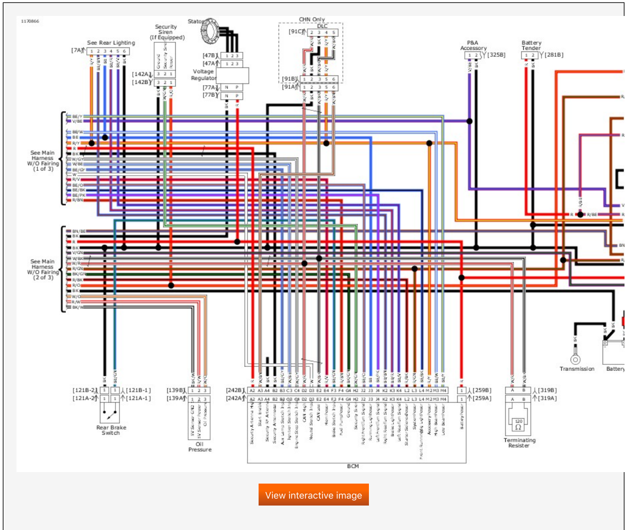
Main Harness (3 of 3): 2019 Touring (without Fairing)
