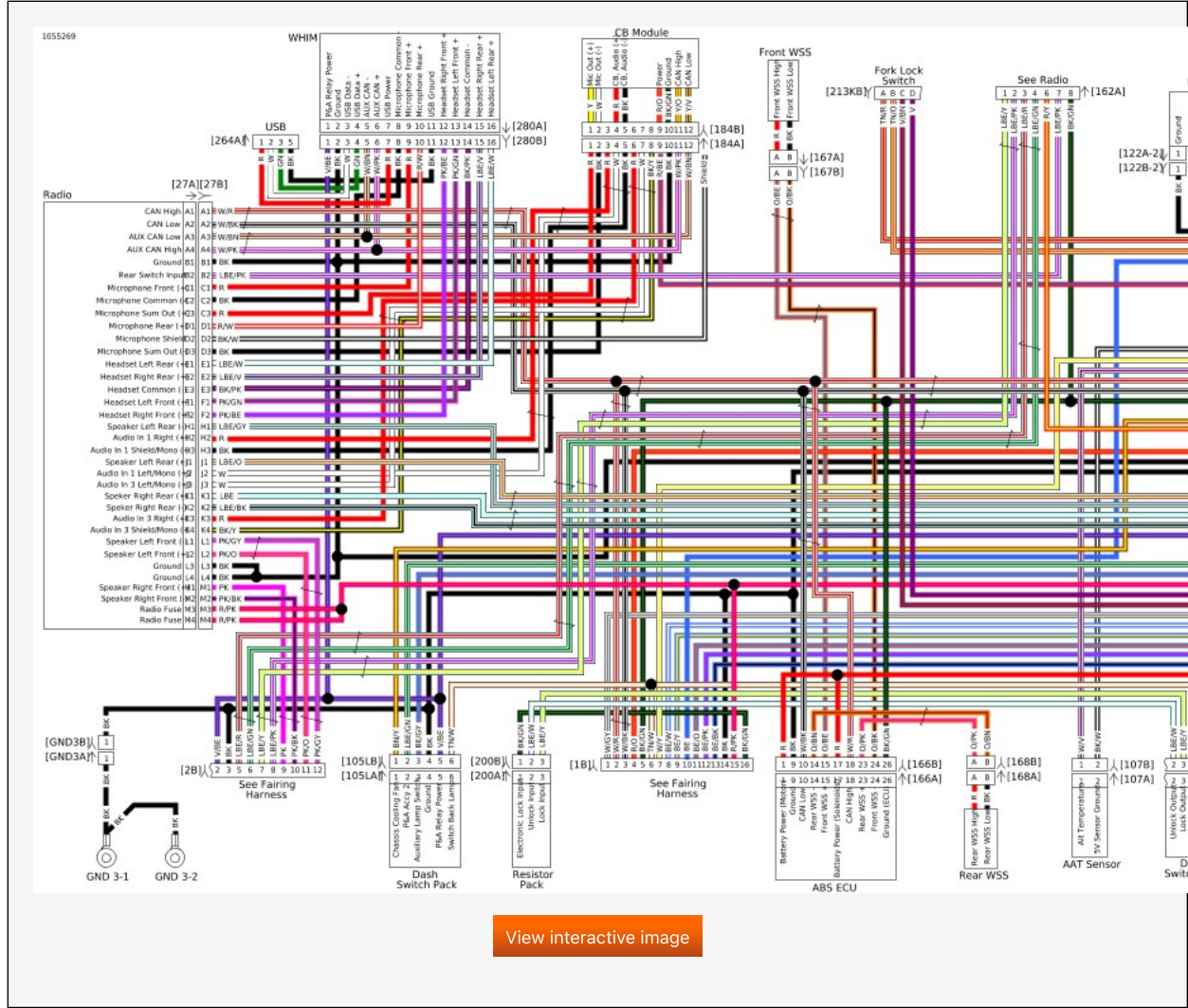
Main Harness (1 of 4): 2019 FLHTKSE
