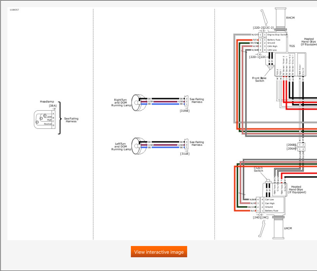
Front Lighting and Hand Controls: 2019 FLHXSE
