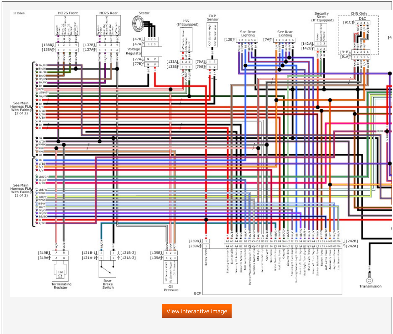
Main Harness FLH (3 of 3): 2019 Touring (with Fairing)
