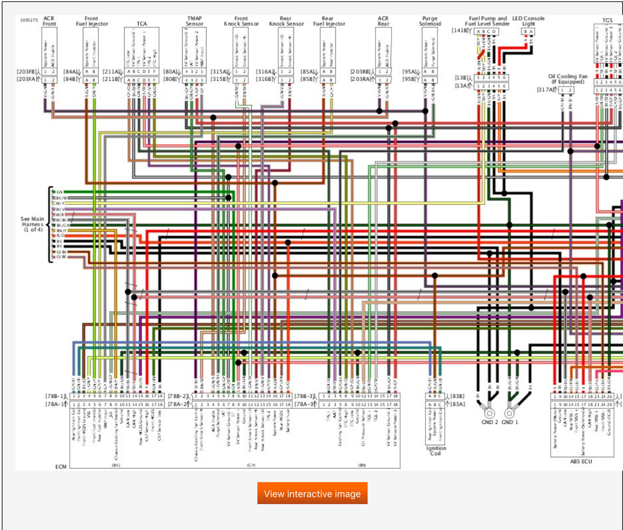
Main Harness (2 of 4): 2019 FTRXSE
