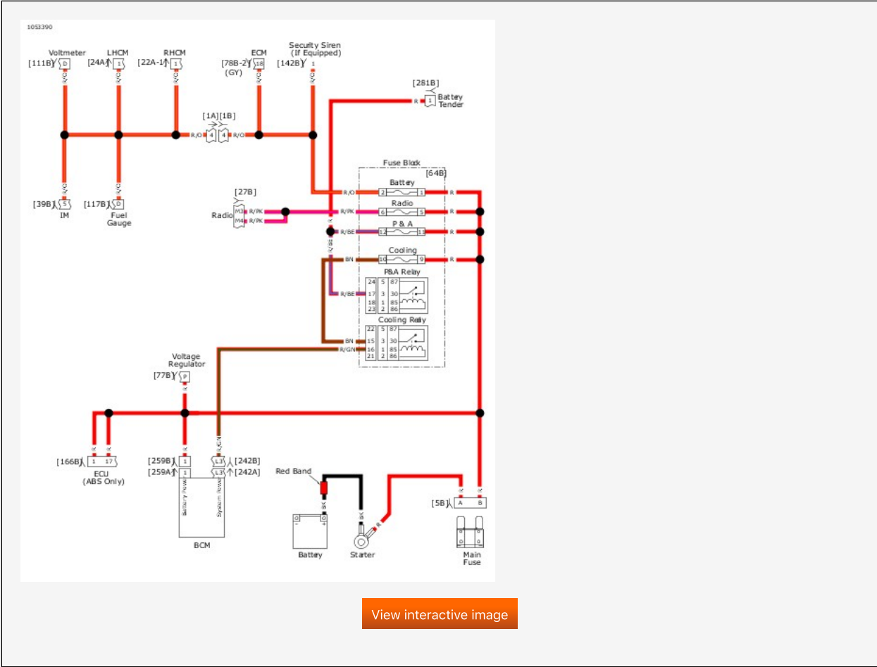
Battery Power Distribution: FLH with Fairing
