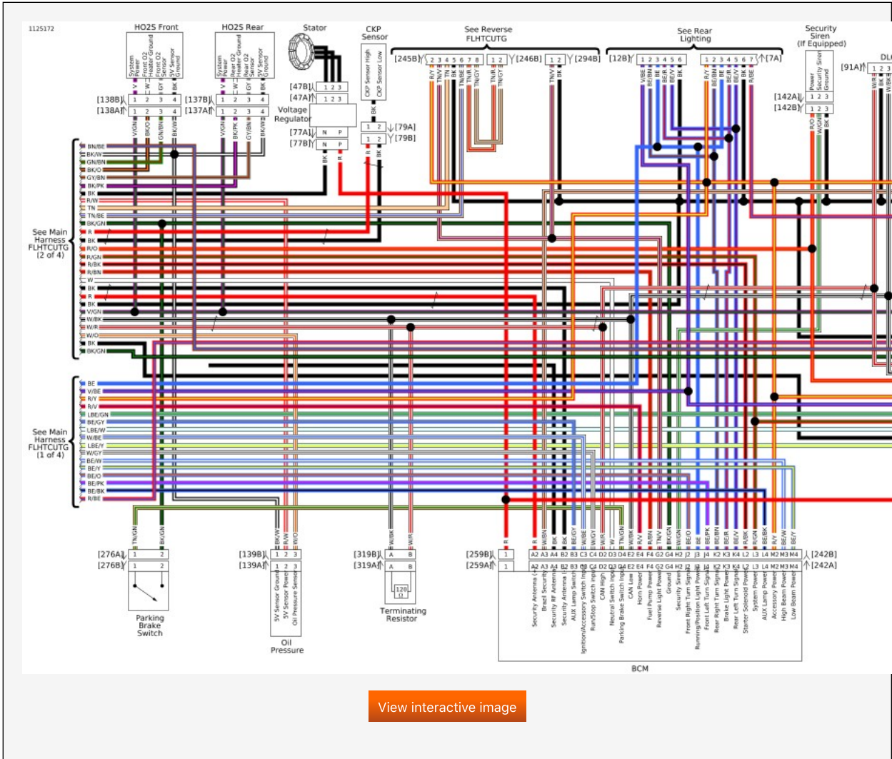
Main Harness FLHTCUTG (3 of 4): 2019 Trike Model
