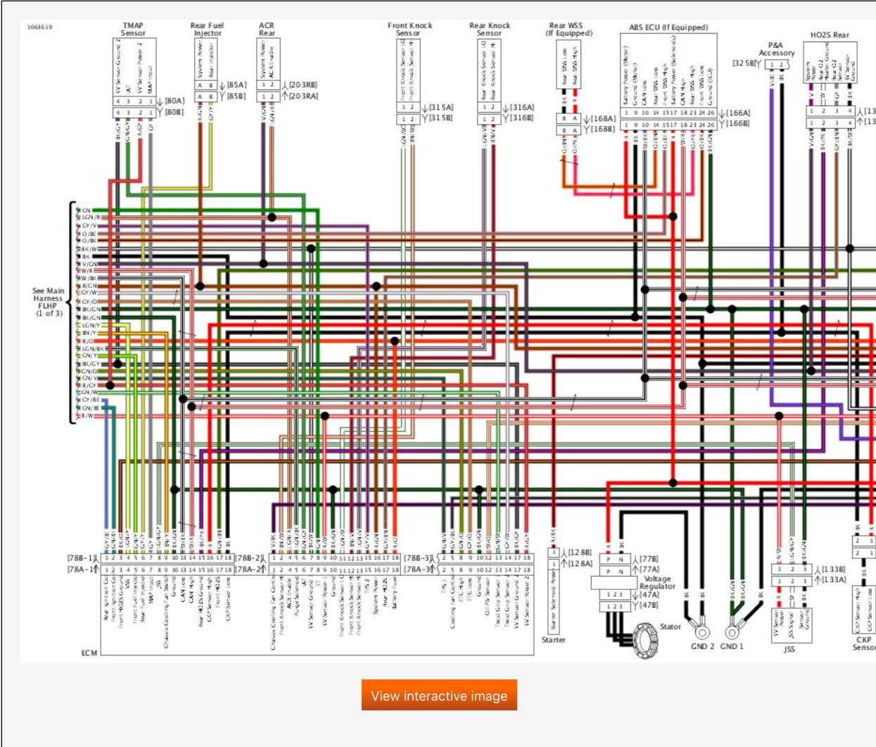
Main Harness (2 of 3): 2019 FLHP
