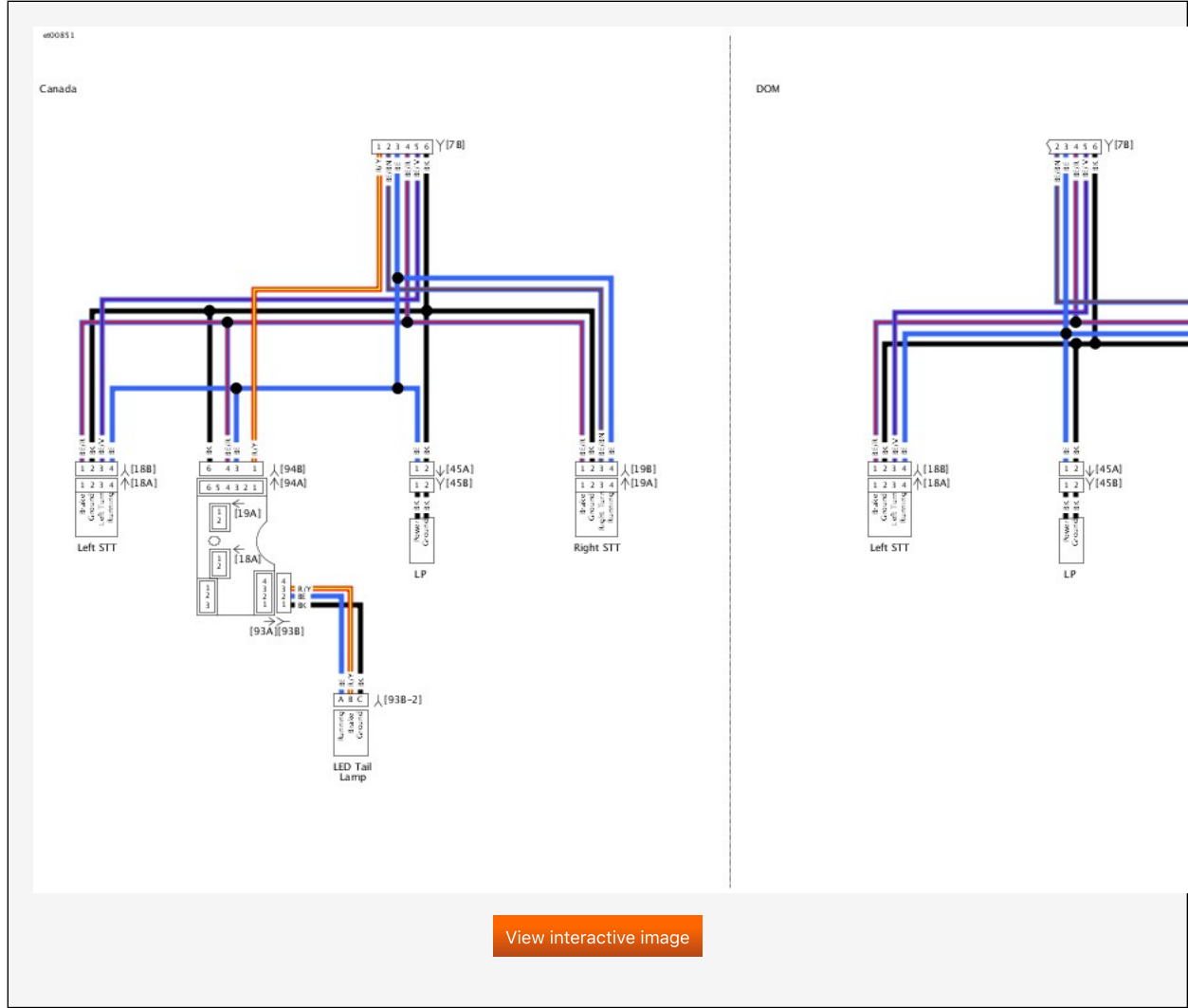
Rear Lighting: 2019 FLTRXSE
