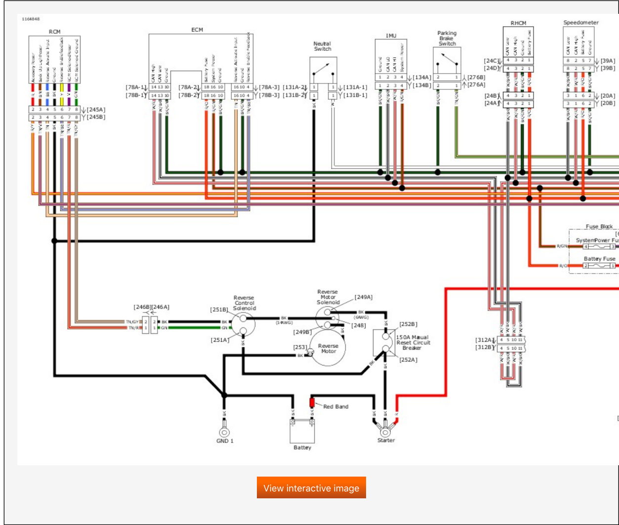
Reverse FLRT: 2019 Trike Model
