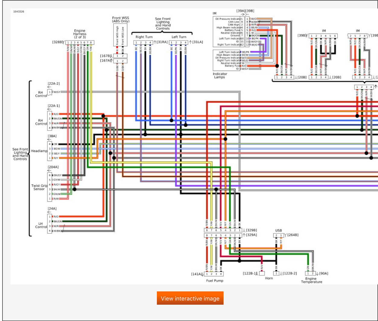
Backbone Harness 1 of 3: 2019 Softail
