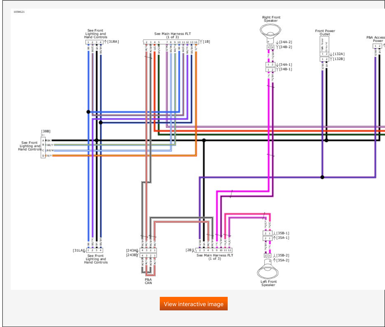
Fairing Harness FLT: 2019 Touring
