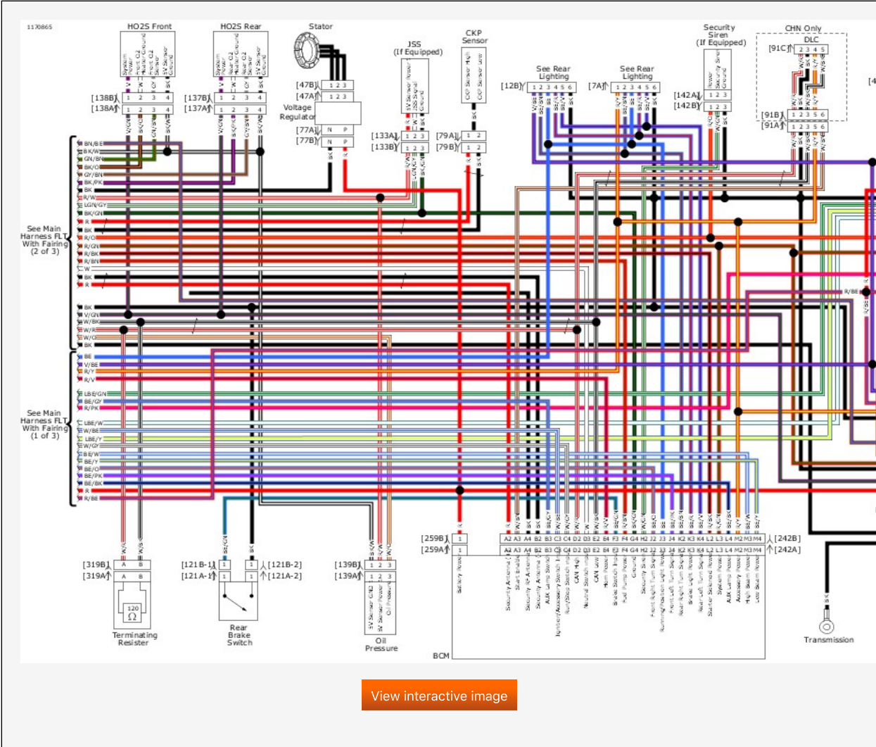
Main Harness FLT (3 of 3): 2019 Touring (with Fairing)
