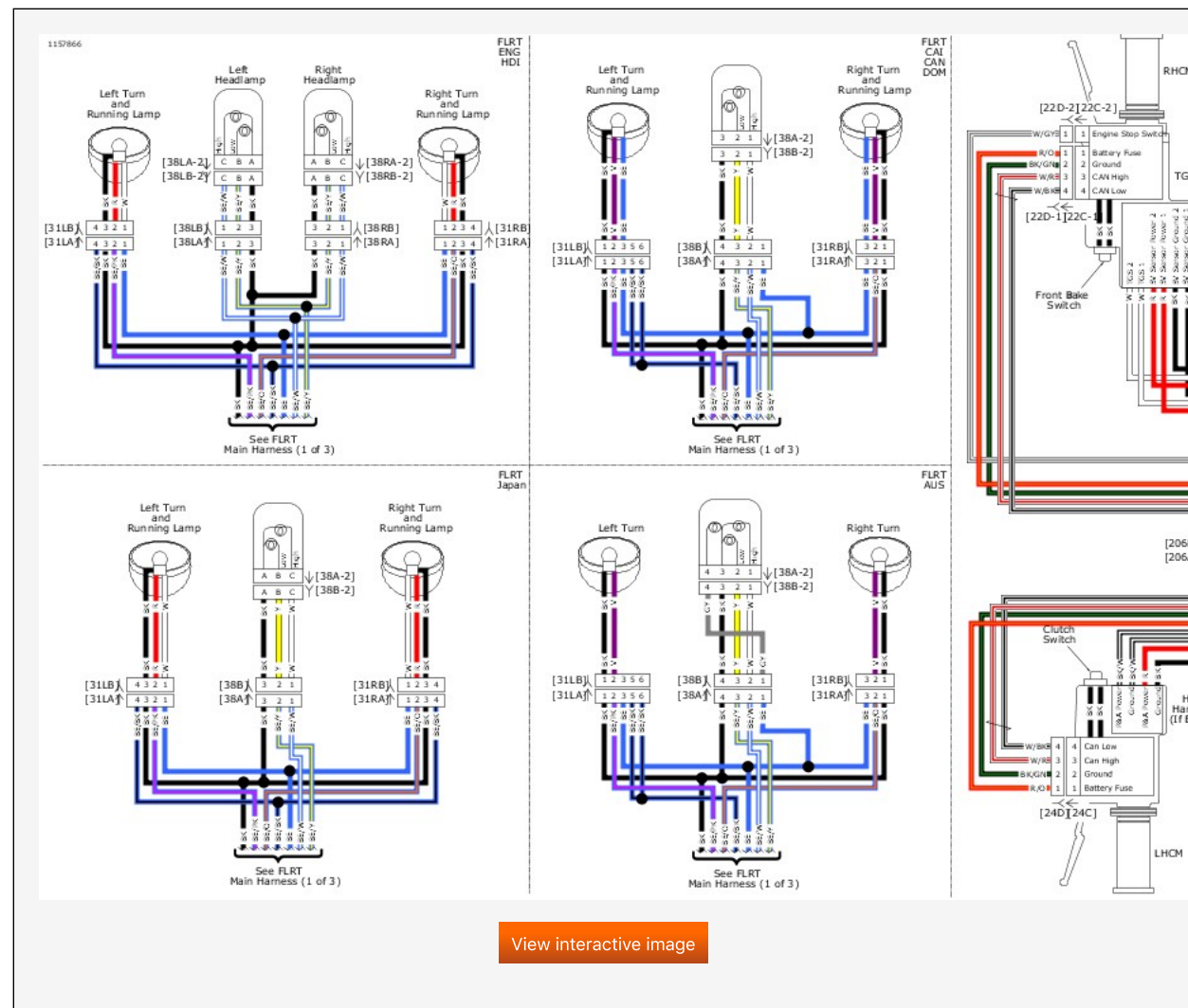
Front Lighting and Hand Controls FLRT: 2019 Trike Model
