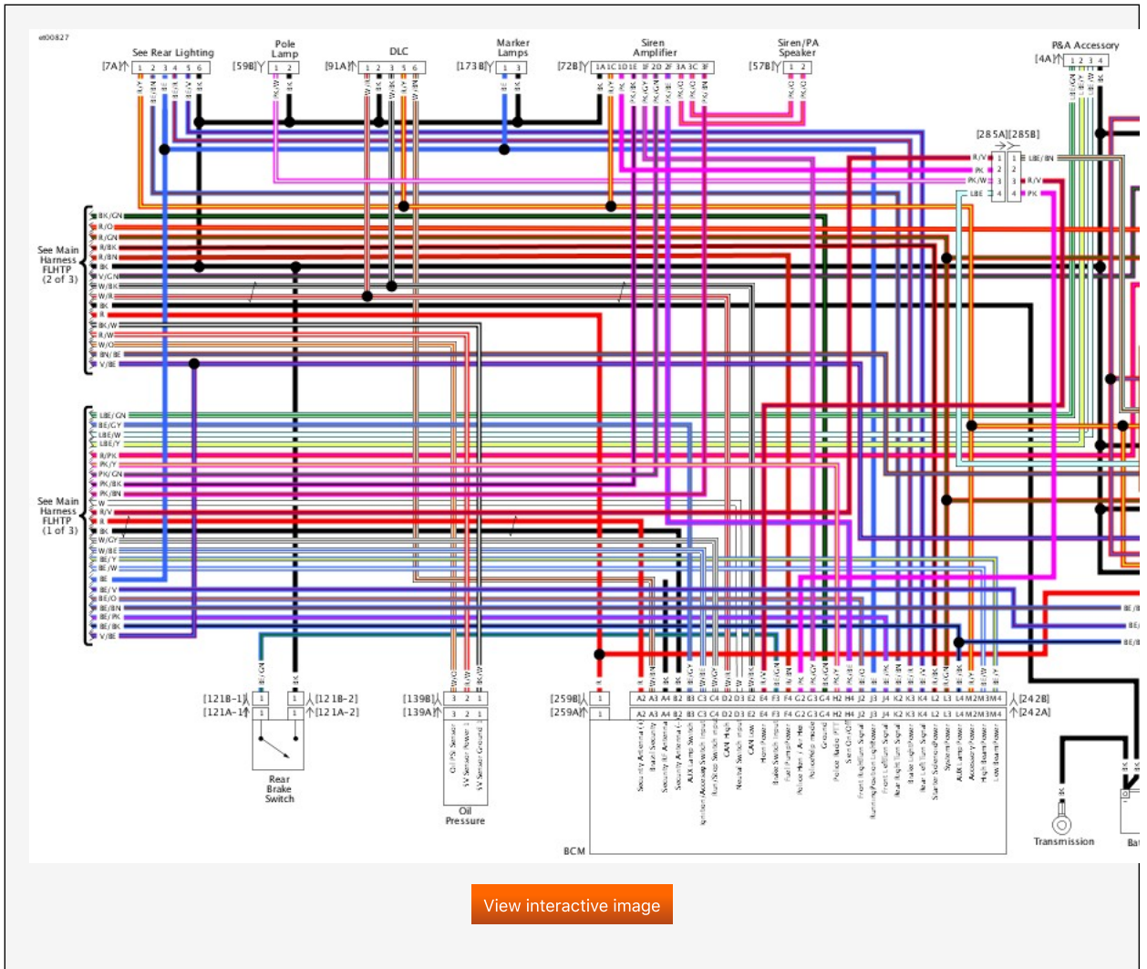
Main Harness (3 of 3): 2019 FLHTP
