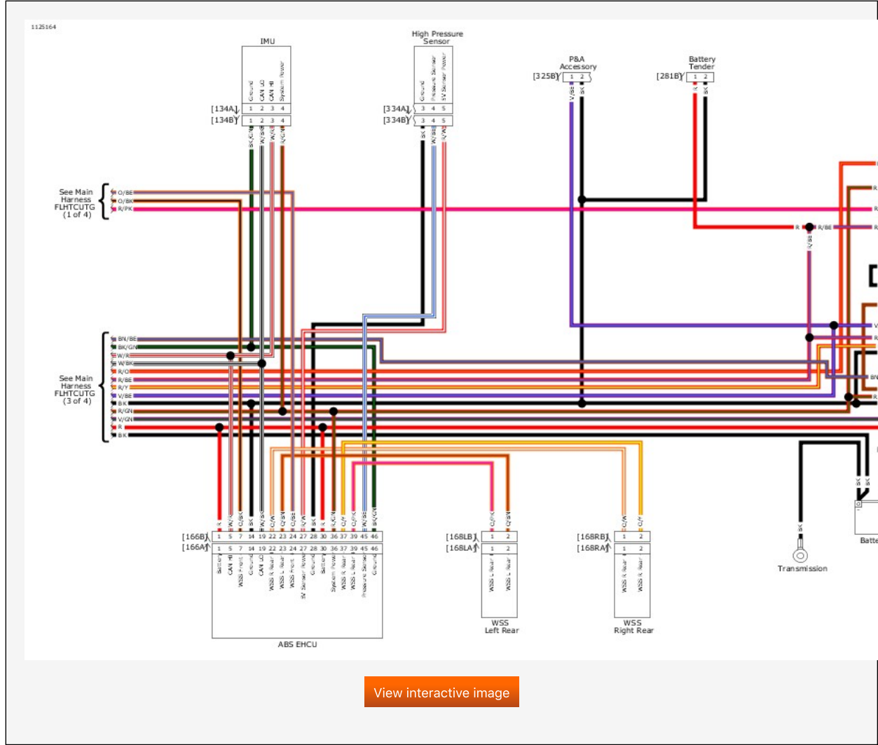
Main Harness FLHTCUTG (4 of 4): 2019 Trike Model
