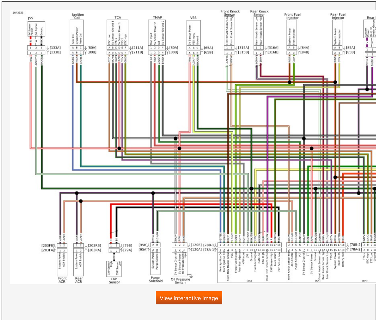
Engine Harness 2 of 3: 2019 Softail
