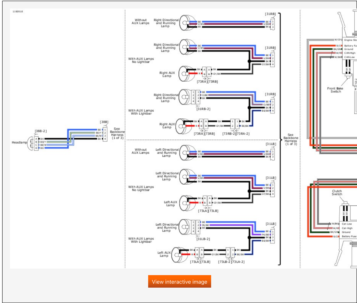
Front Lighting and Hand Controls: 2019 Softail
