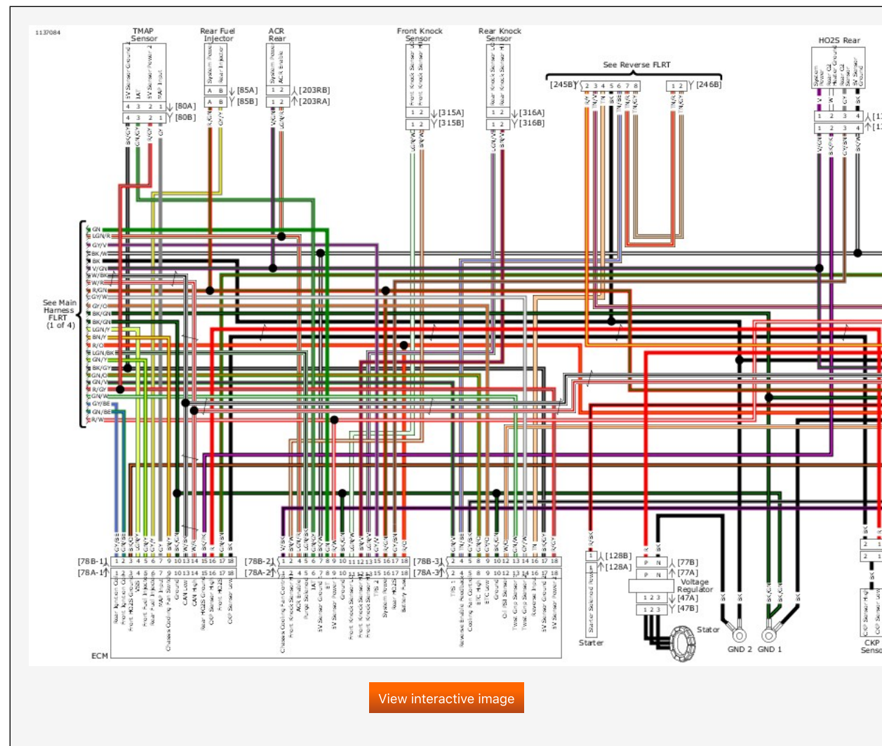
Main Harness FLRT (2 of 4): 2019 Trike Model
