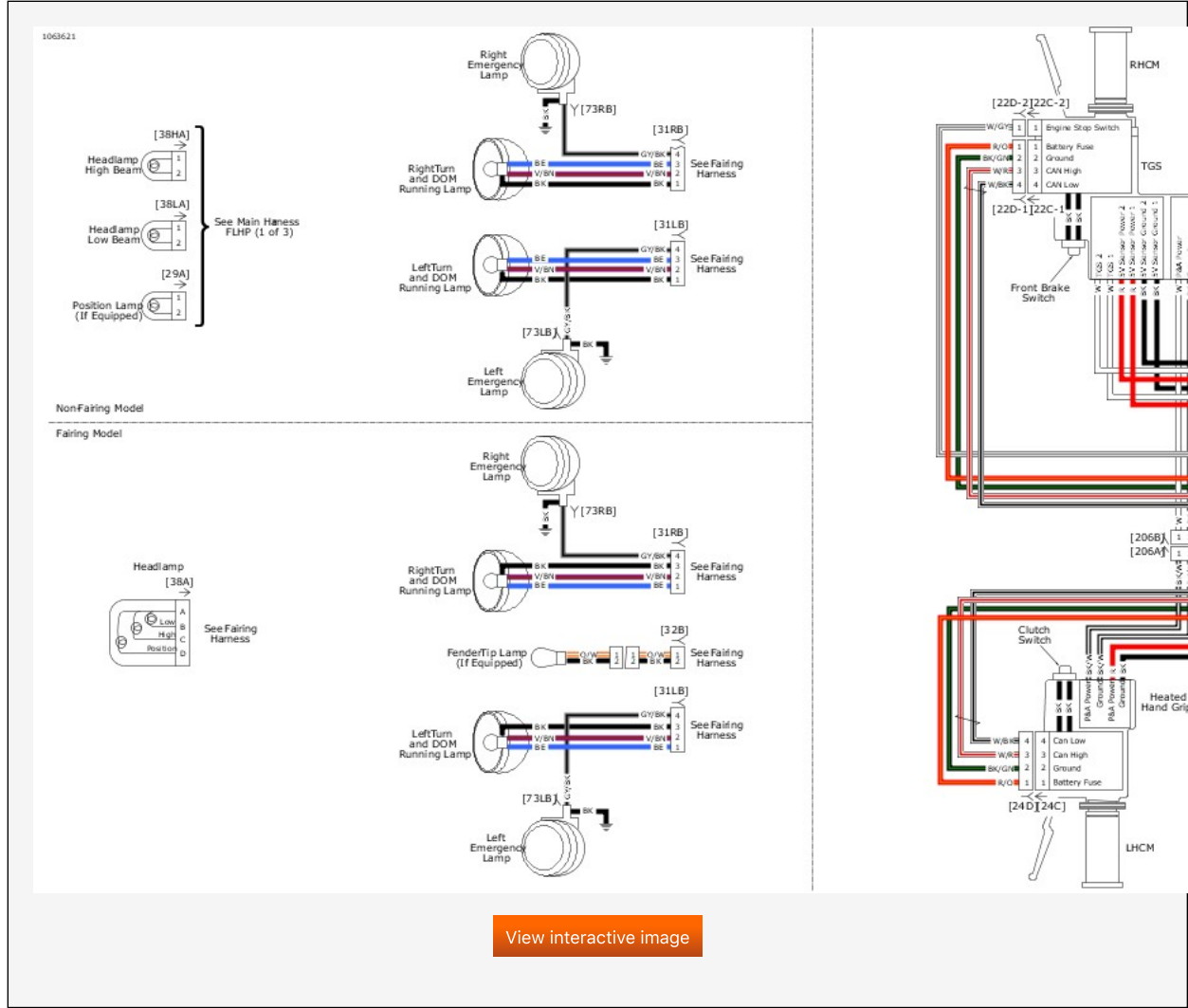
Front Lighting and Hand Controls: 2019 Police
