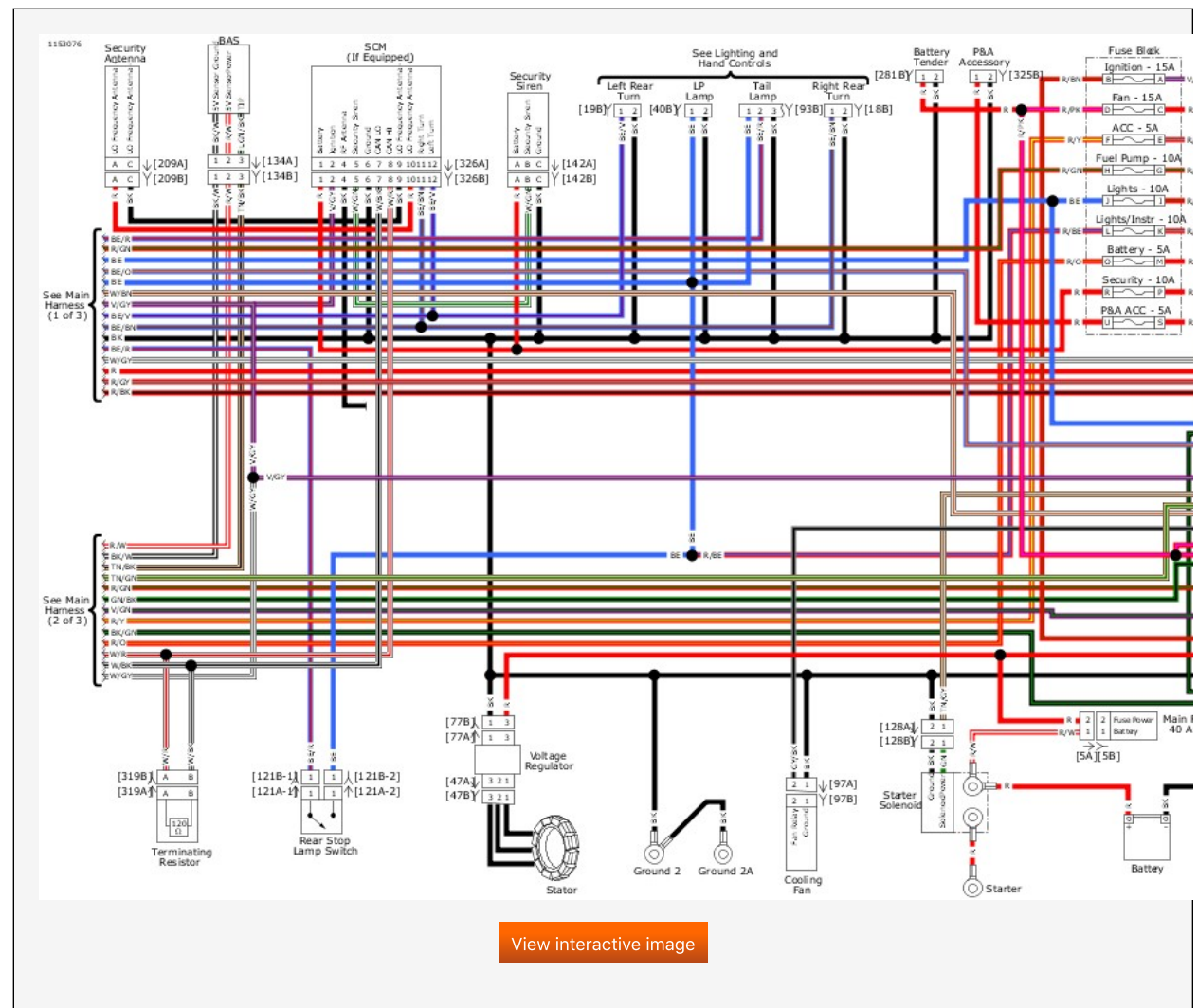
Main Harness (3 of 3) (750A): 2019 Street
