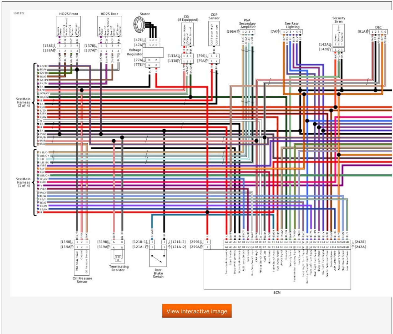
Main Harness (3 of 4): 2019 FLHTKSE
