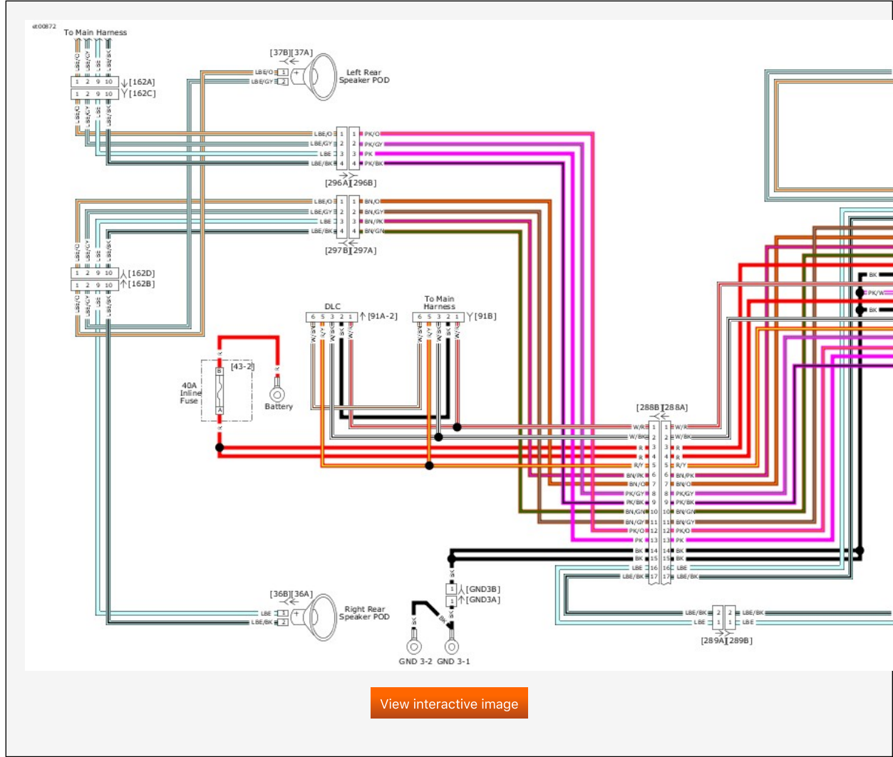
P&A Radio with 2 Amps (2 of 2): 2019 Touring
