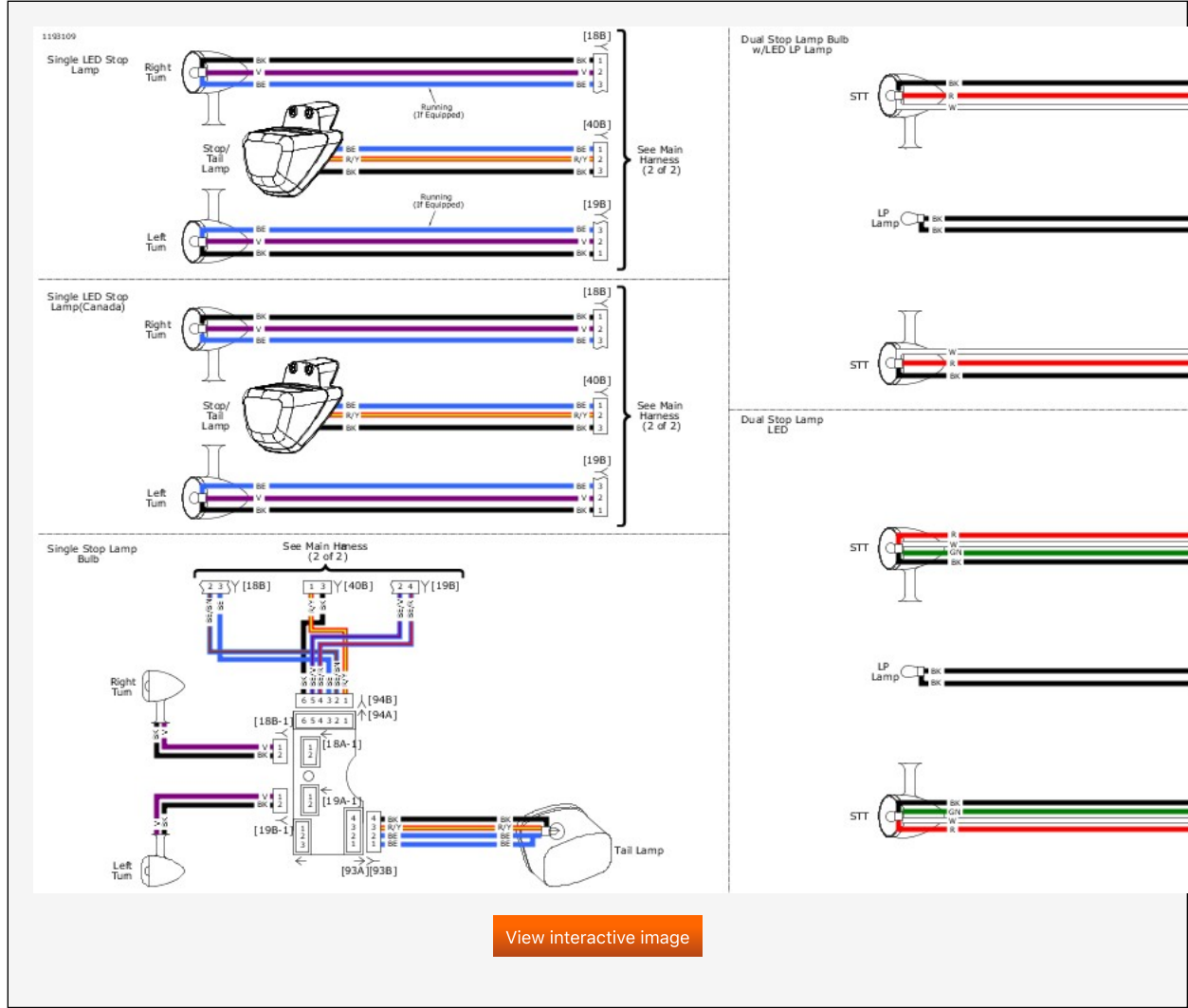
Rear Lighting: 2019 Sportster
