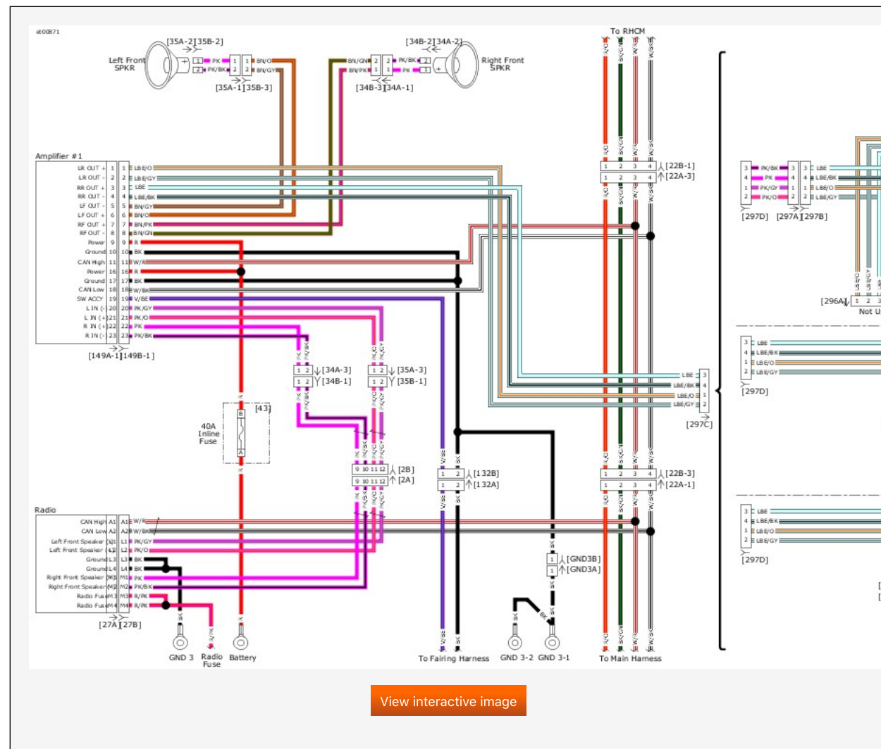
P&amp;A Radio with 1 Amp: 2019 Touring
