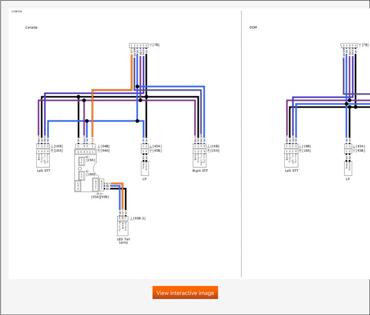
Rear Lighting: 2019 FLHXSE
