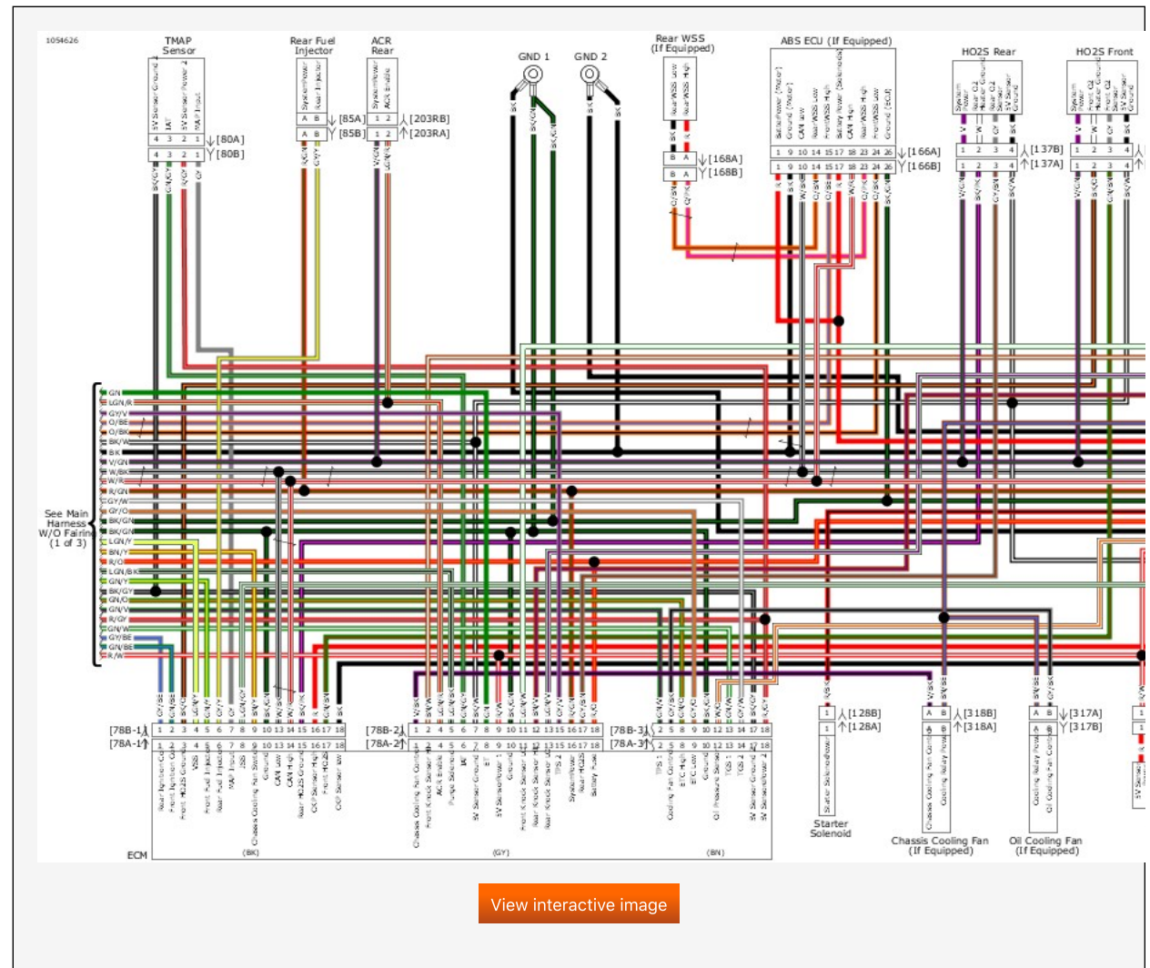
Main Harness (2 of 3): 2019 Touring (without Pairing)
