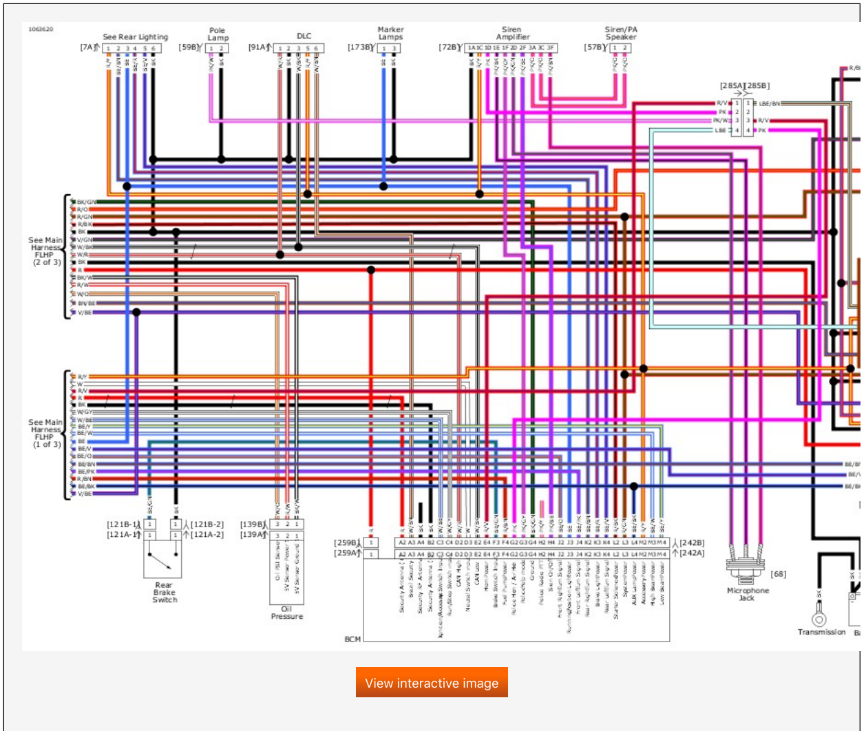
Main Harness (3 of 3): 2019 FLHP
