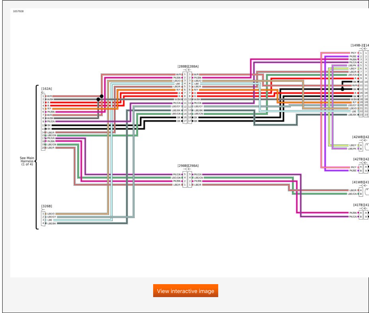
Radio (2 of 2): 2019 FLTRXSE
