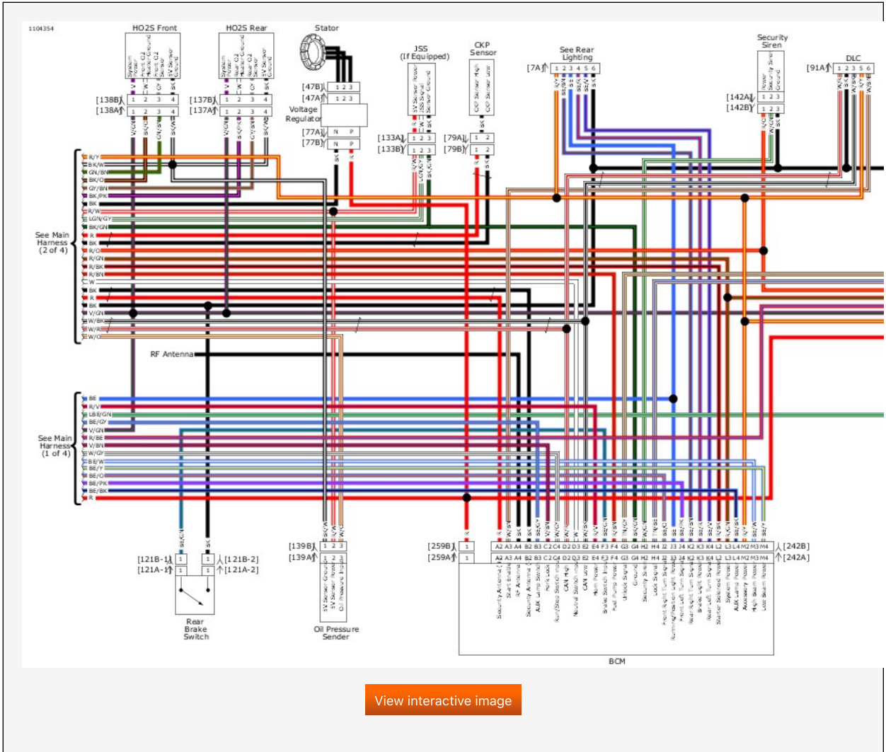
Main Harness (3 of 4): 2019 FLHXSE
