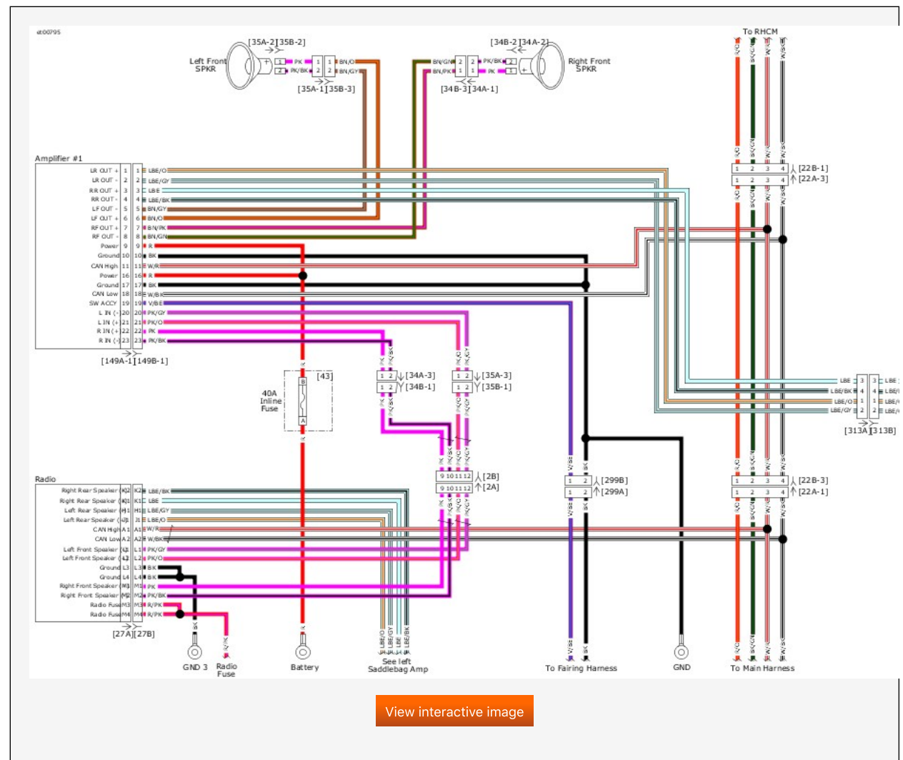
P&amp;A Radio with 4 Amps (1 of 4), Front Amp: 2019 Touring
