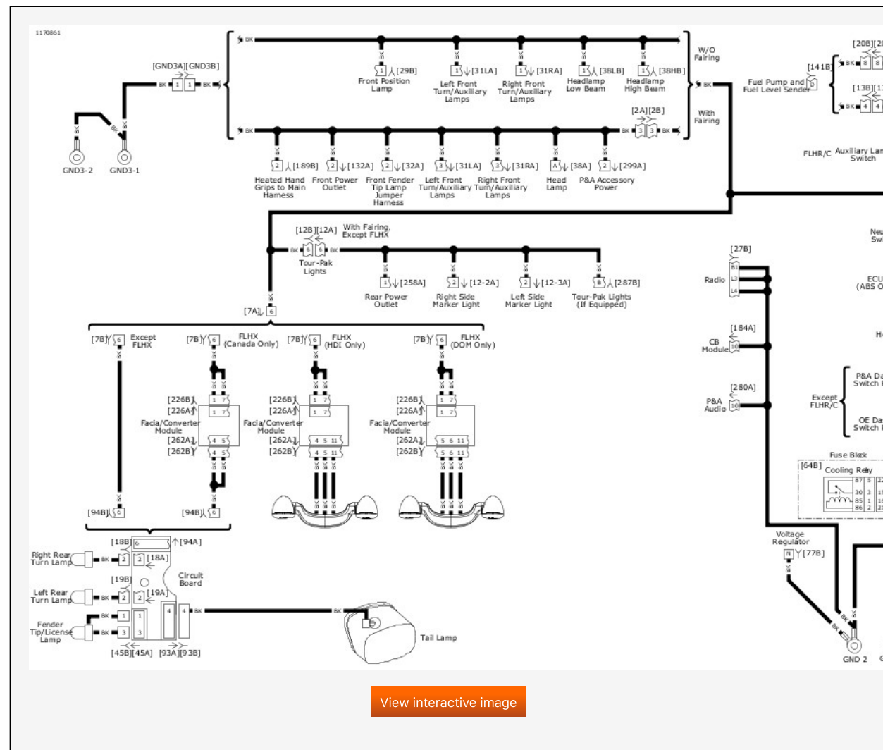
Ground Circuit FLH: 2019 Touring
