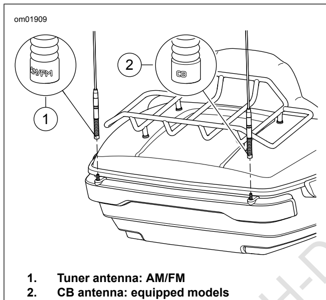
Figure 32. Antennas
