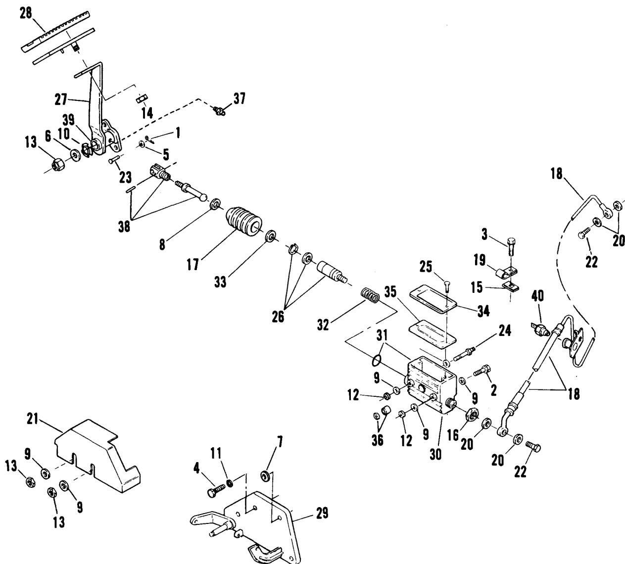
REAR BRAKE CONTROL — FLST
