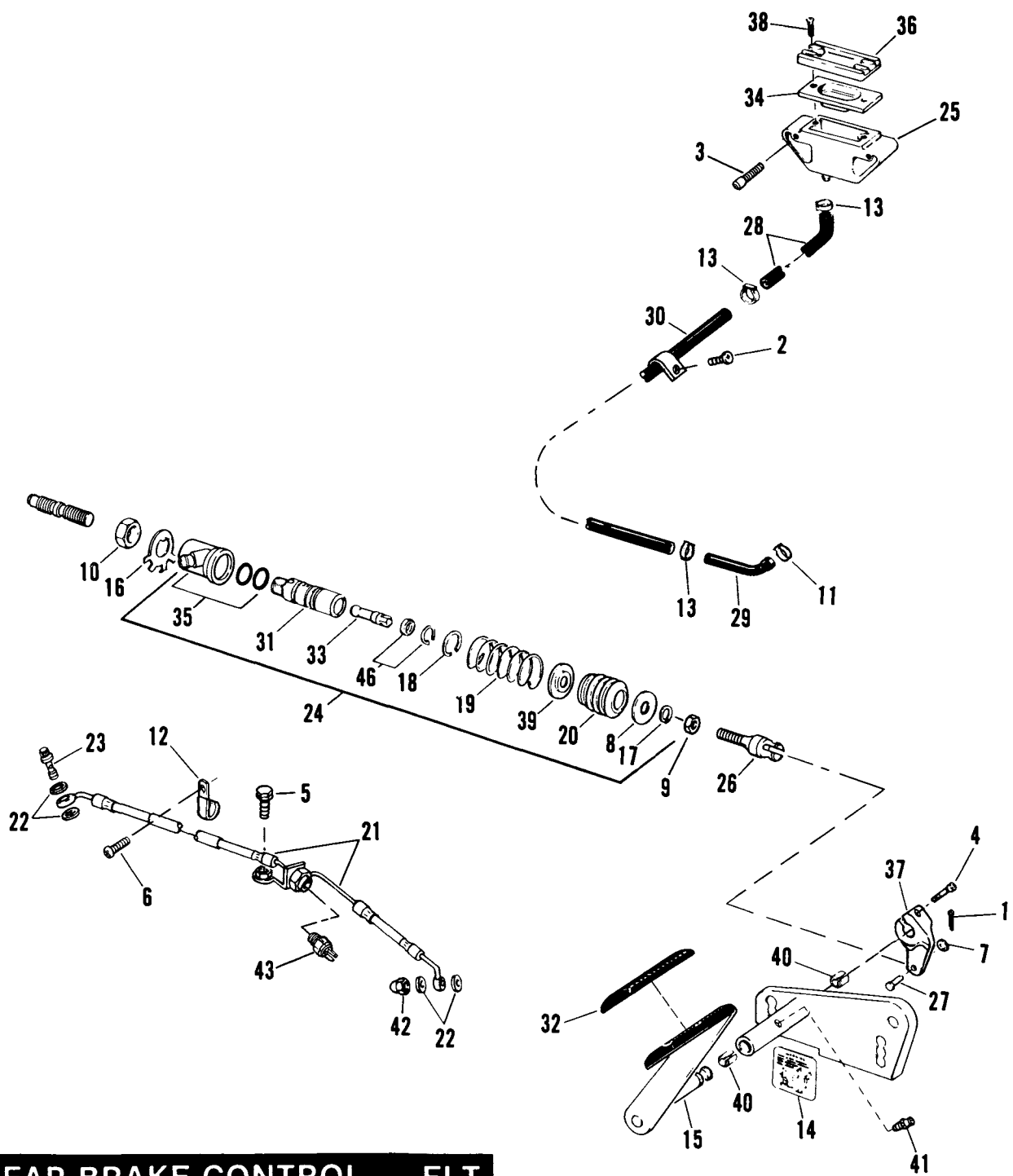
REAR BRAKE CONTROL — FLT
