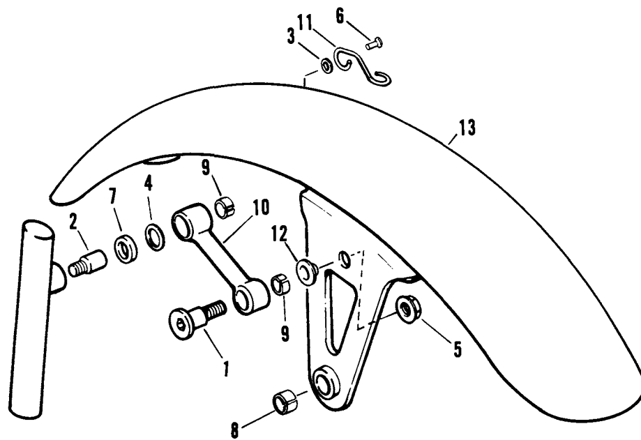
FRONT FENDER – FXSTS
