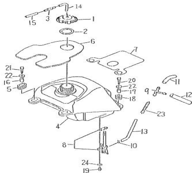
FIG 20 FUEL TANK
