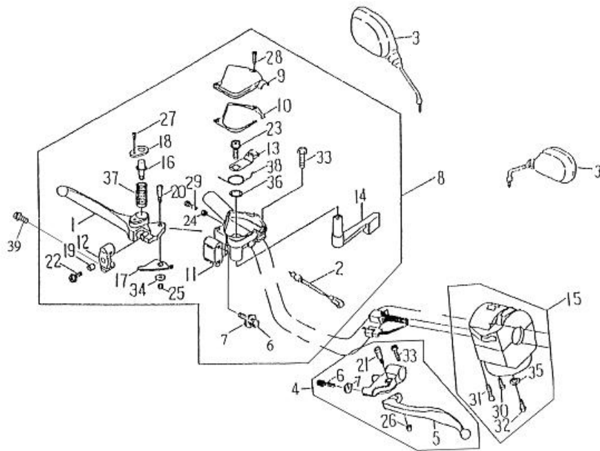
FIG 29 HANDLE SWITCH,LEVER
