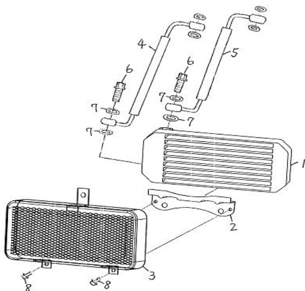
FIG 39 OIL COOLING SET
