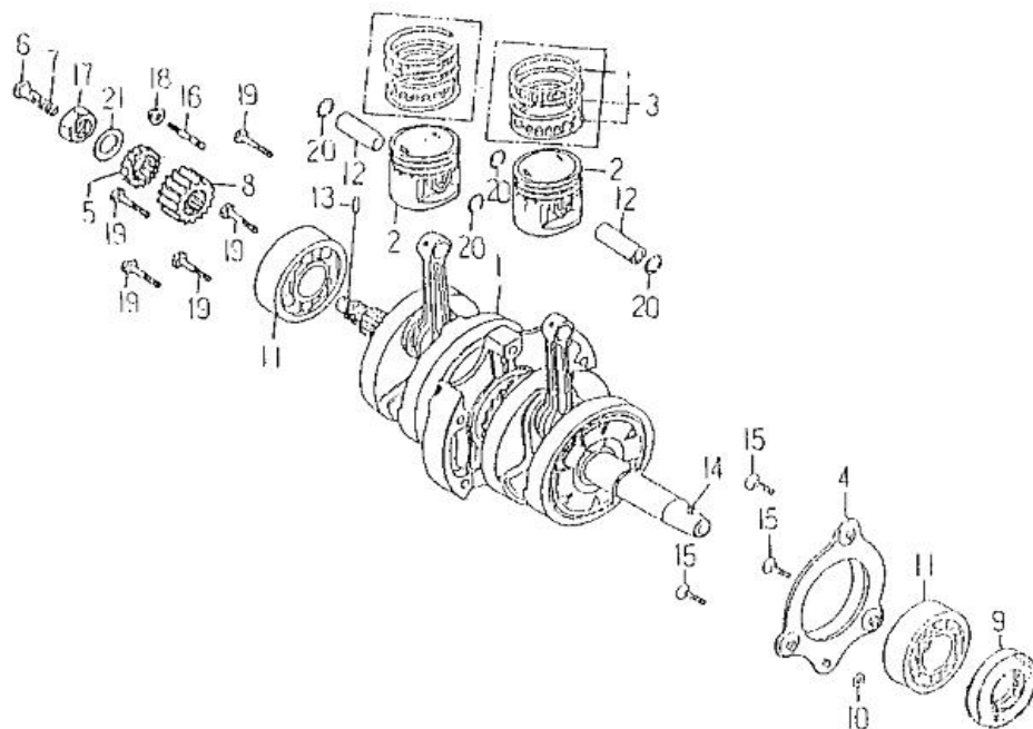
FIG 02 CRANKSHAFT.PISTON
