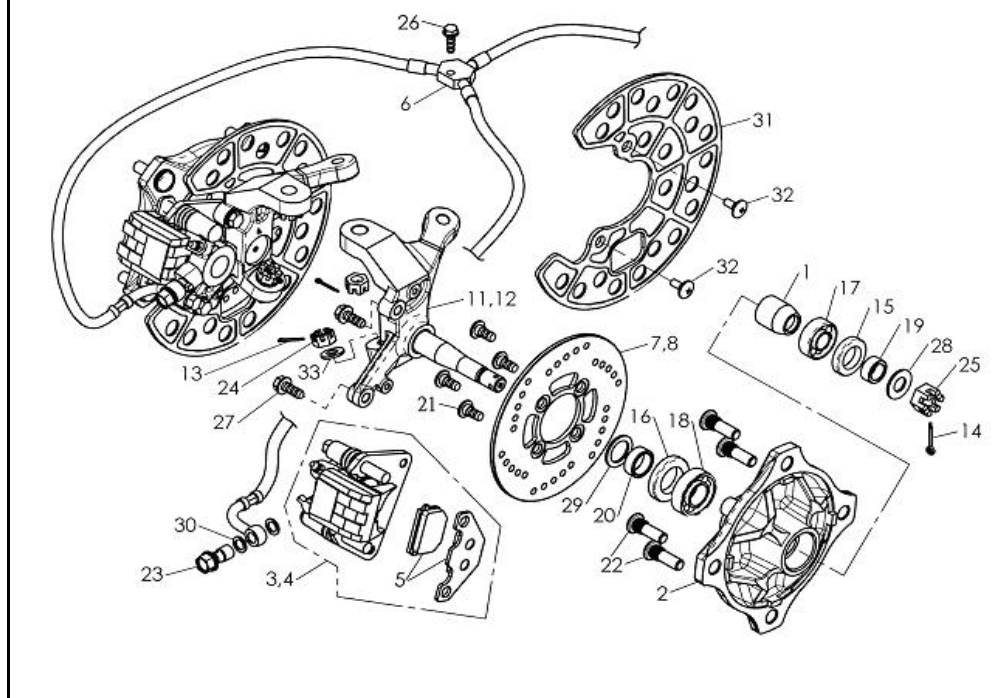
FIG 25 FRONT BRAKE
