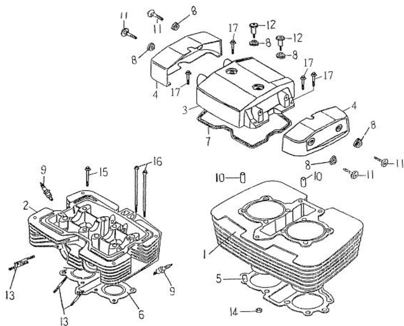
FIG 01 CYLINDER.CYLINDER HEAD
