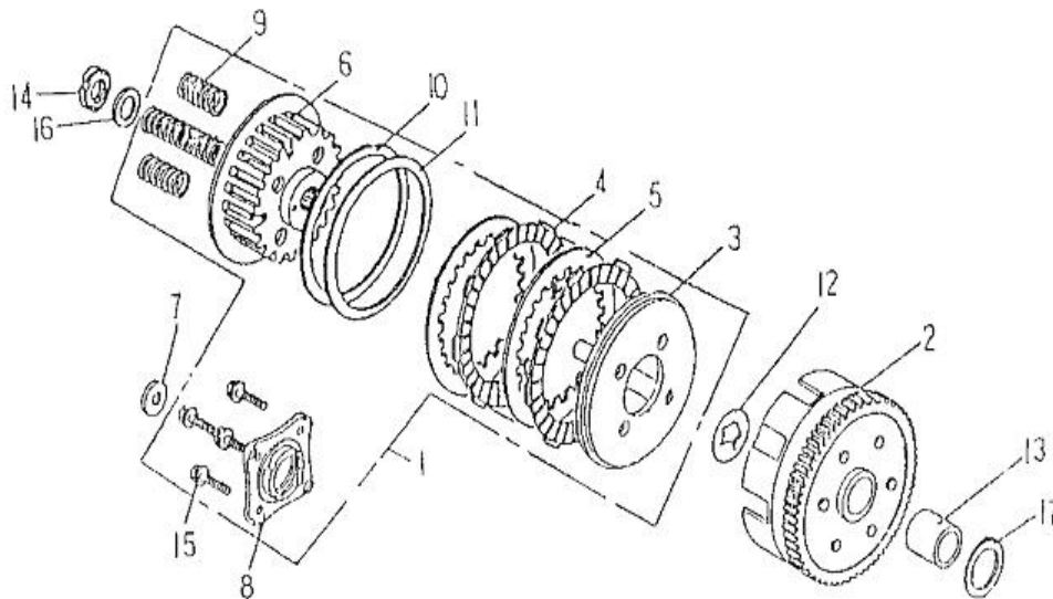
FIG 13 CLUTCH
