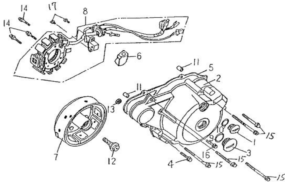
FIG 08 LEFT CRANKCASE COVER
