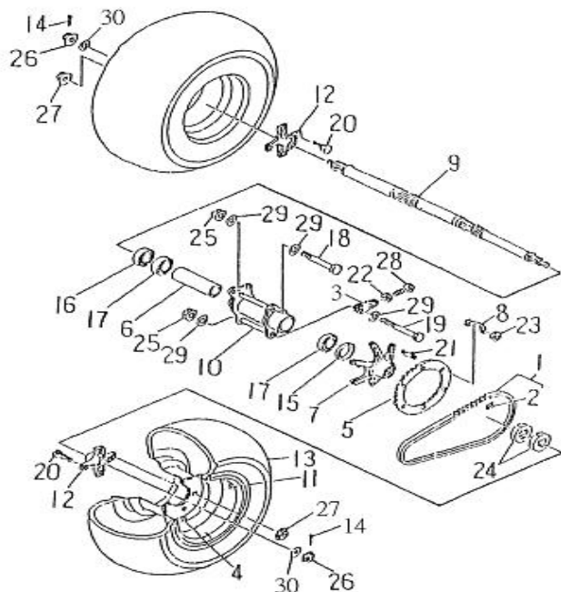
FIG 26 REAR WHEEL
