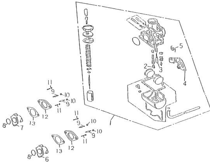
FIG 04 CARBURETOR
