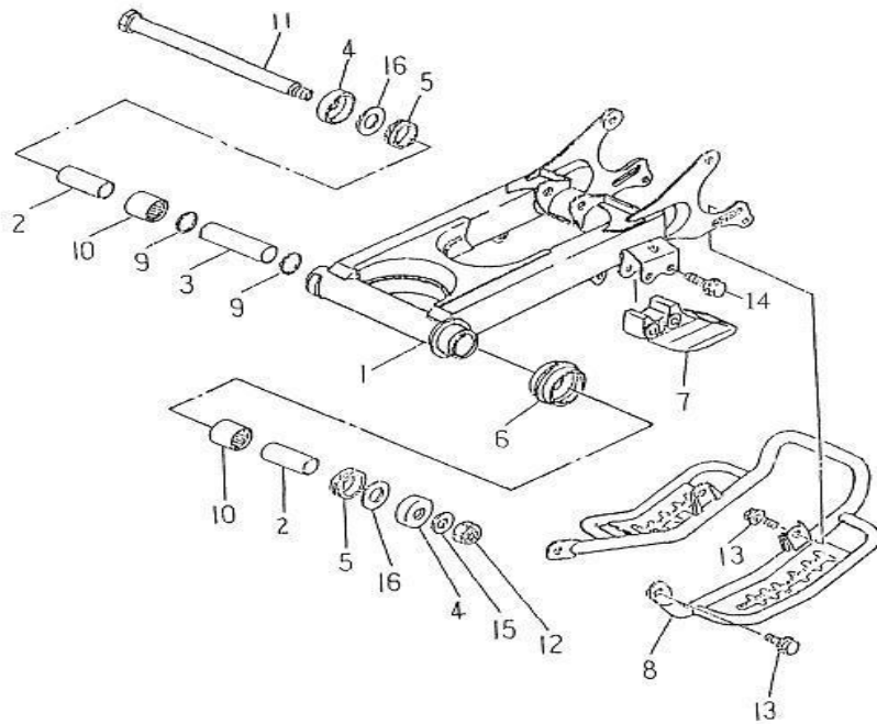
FIG 15 REAR ARM
