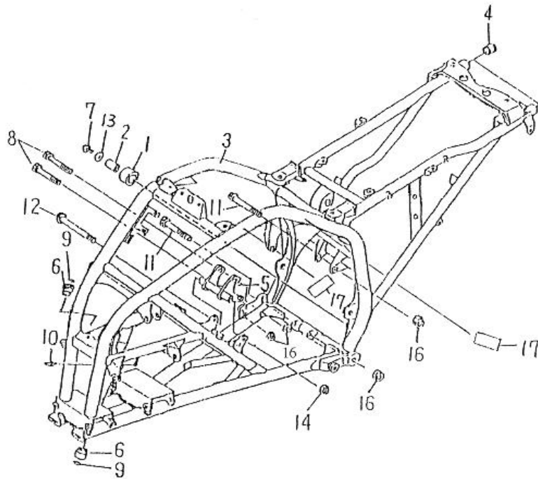
FIG 17 FRAME
