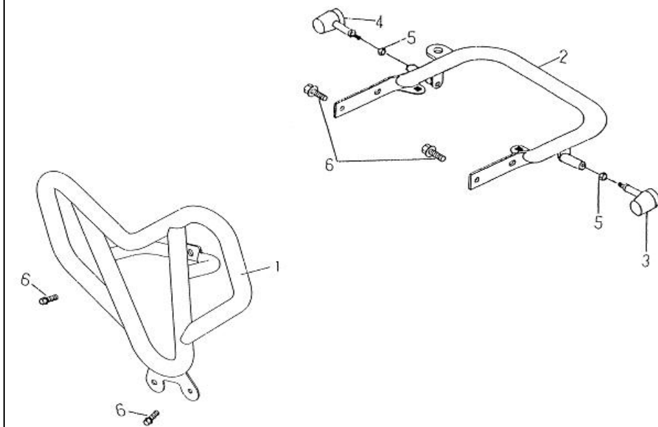
FIG 31 GUARD
