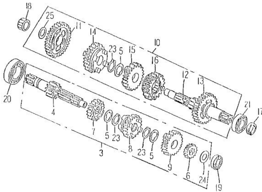
FIG 10 TRANSMISSION STARTER
