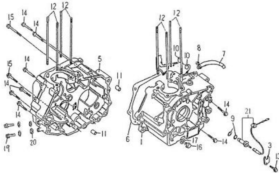
FIG 07 CRANKCASE
