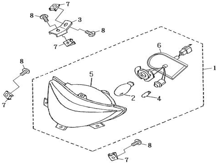
FIG 32 HEAD LIGHT
