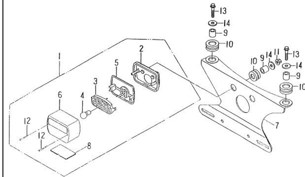
FIG 33 TAIL LIGHT
