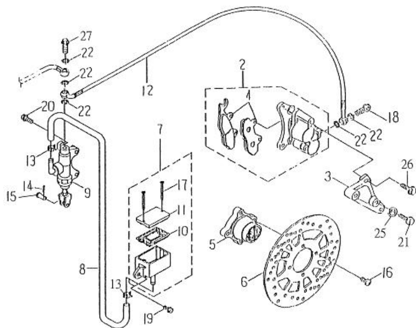
FIG 27 REAR BRAKE
