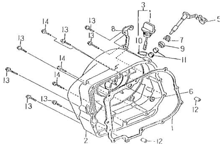
FIG 09 RIGHT CRANKCASE COVER
