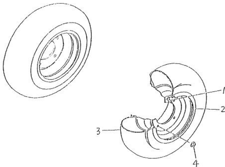
FIG 24 FRONT WHEEL
