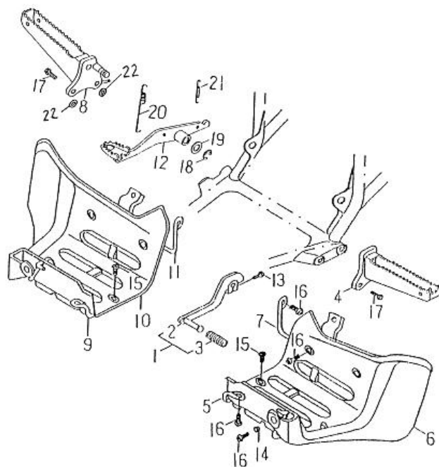
FIG 30 FOOTREST
