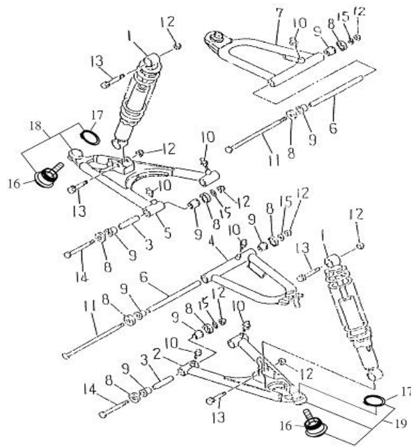
FIG 18 FRONT SUSPENSION
