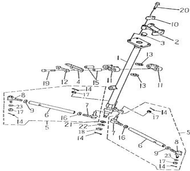
FIG 19 STEERING
