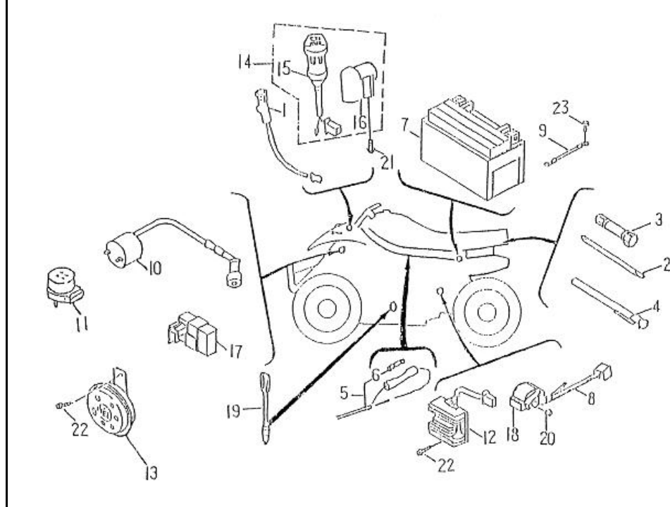
FIG 34 WIRE HARNESS
