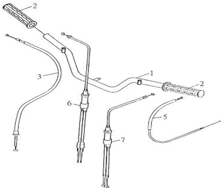
FIG 28 STEERING HANDLE CABLE
