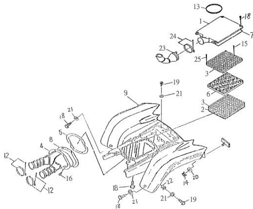
FIG 22 SIDE COVER
