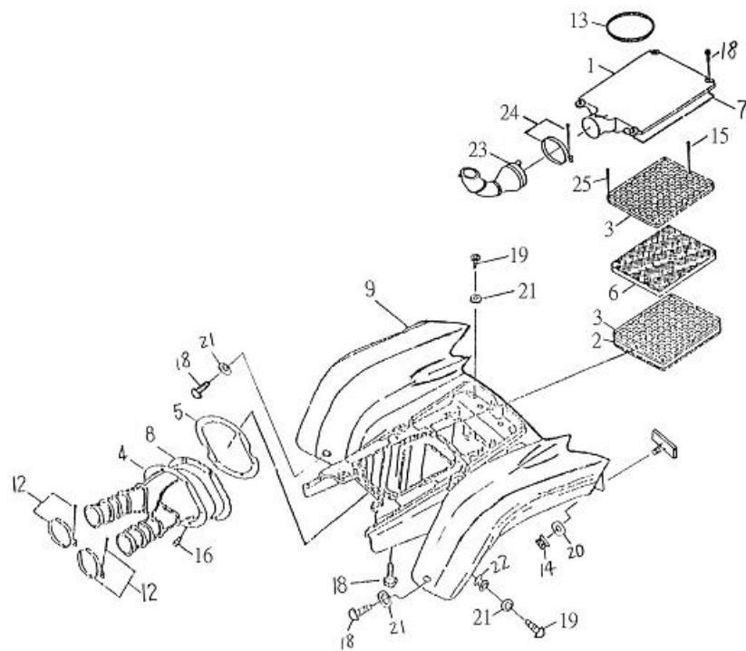
FIG 22 SIDE COVER
