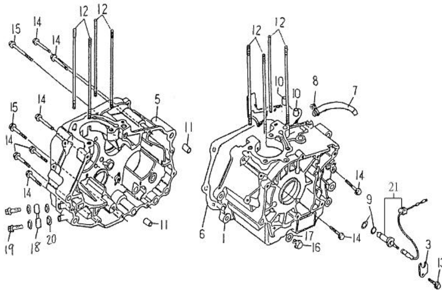
FIG 07 CRANKCASE
