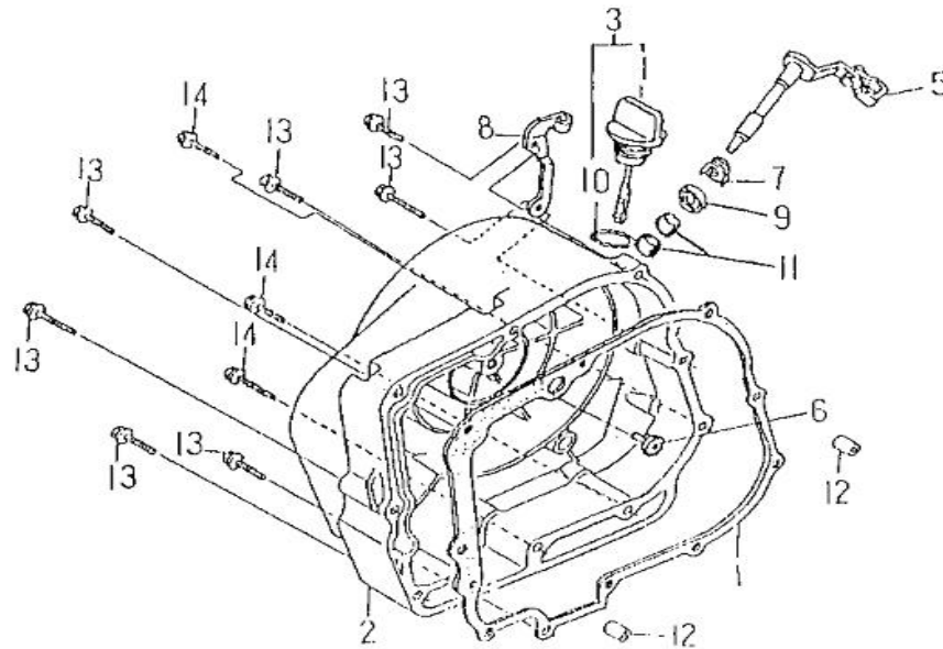
FIG 09 RIGHT CRANKCASE COVER
