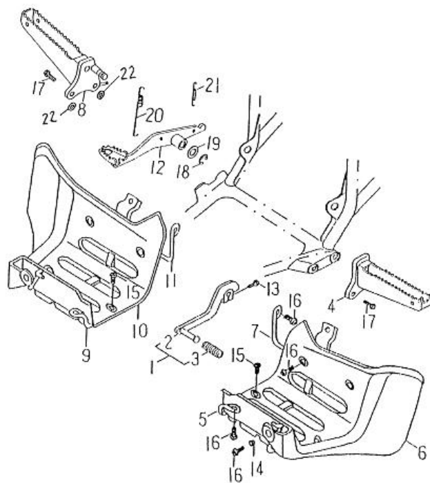
FIG 30 FOOTREST
