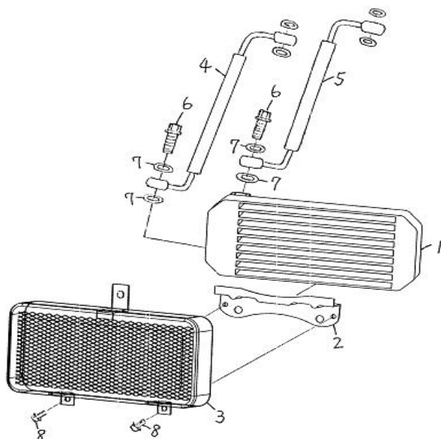
FIG 39 OIL COOLING SET
