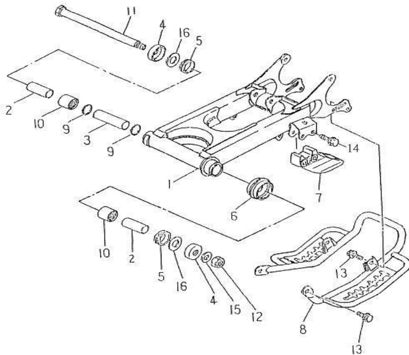
FIG 15 REAR ARM
