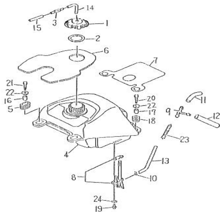
FIG 20 FUEL TANK
