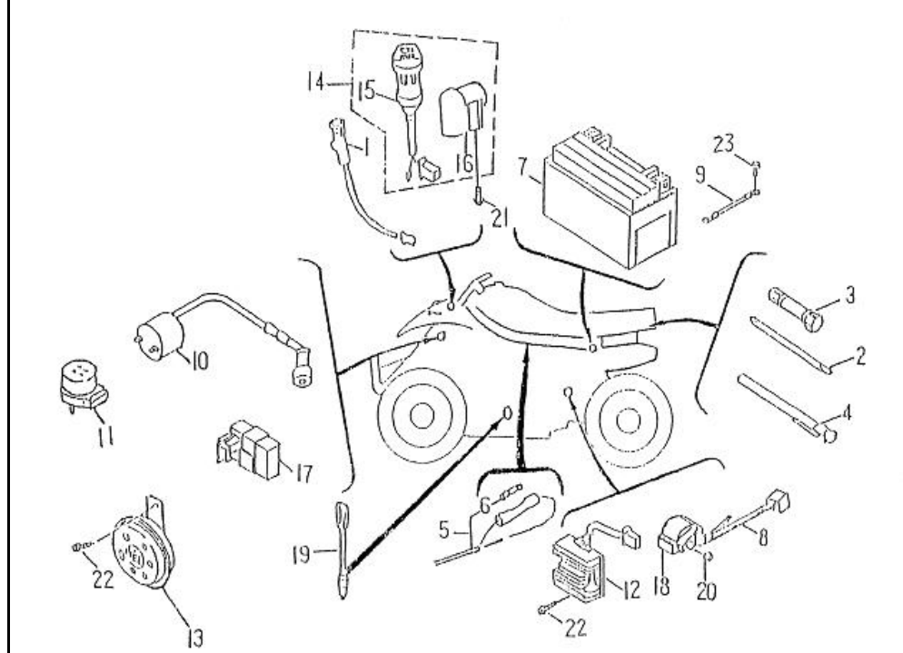
FIG 34 WIRE HARNESS
