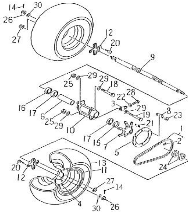
FIG 26 REAR WHEEL
