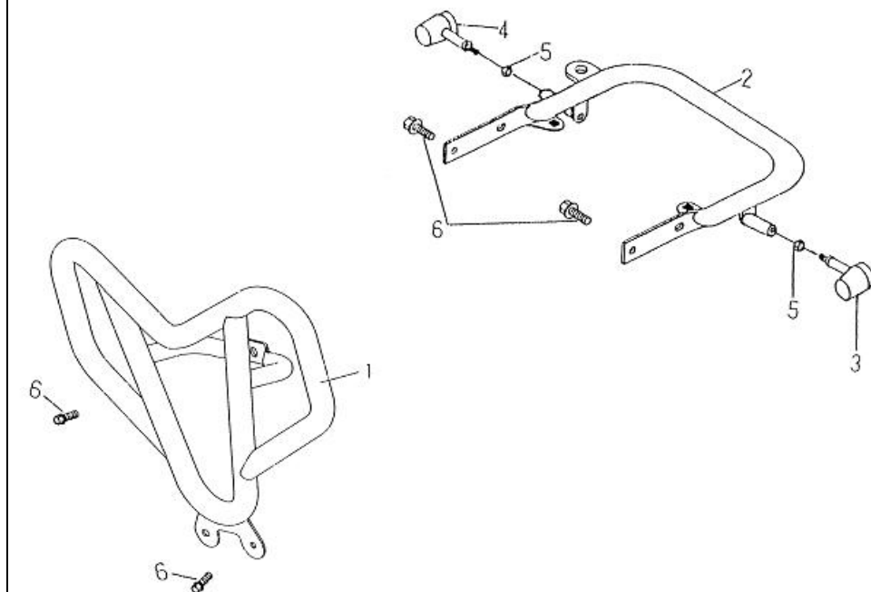
FIG 31 GUARD
