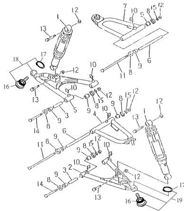
FIG 18 FRONT SUSPENSION
