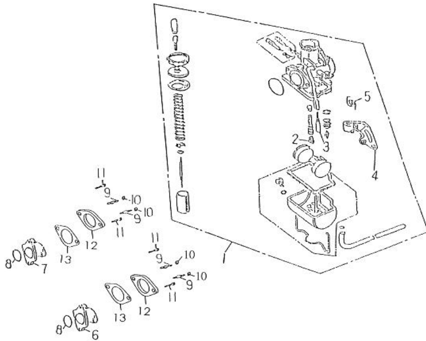
FIG 04 CARBURETOR
