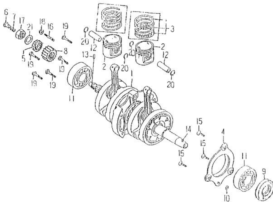
FIG 02 CRANKSHAFT.PISTON
