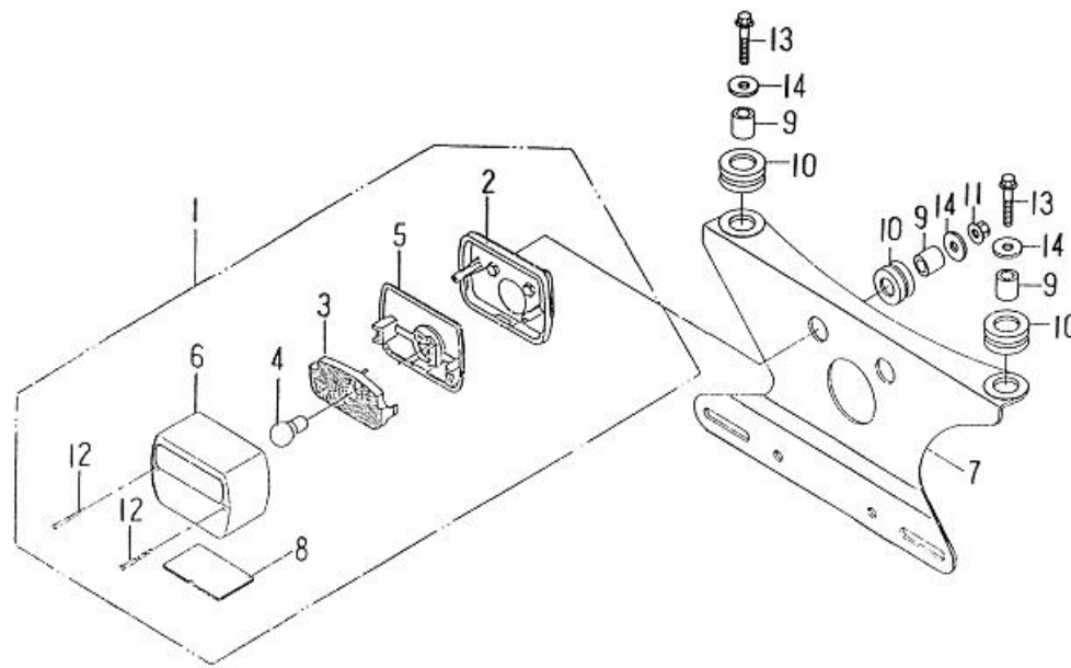
FIG 33 TAIL LIGHT
