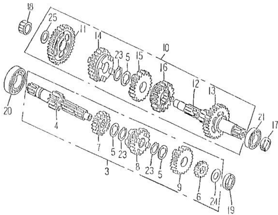
FIG 10 TRANSMISSION STARTER
