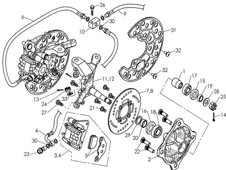
FIG 25 FRONT BRAKE
