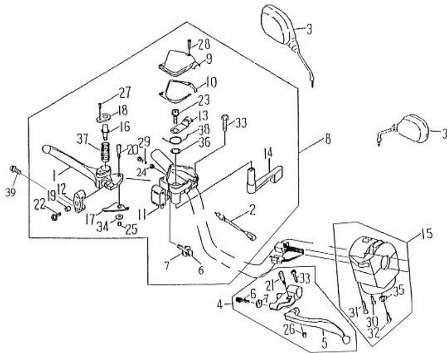
FIG 29 HANDLE SWITCH,LEVER
