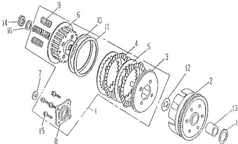
FIG 13 CLUTCH
