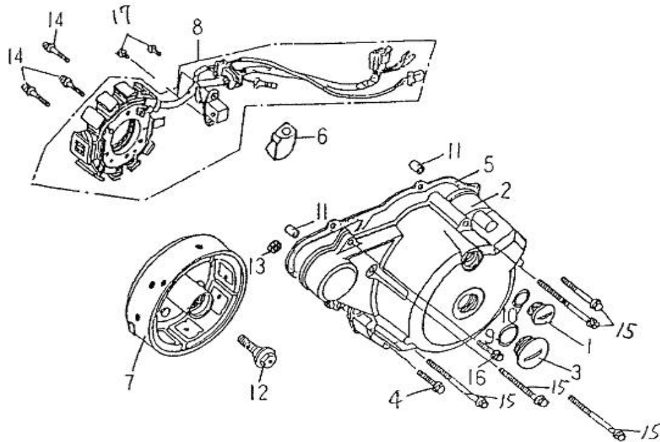
FIG 08 LEFT CRANKCASE COVER
