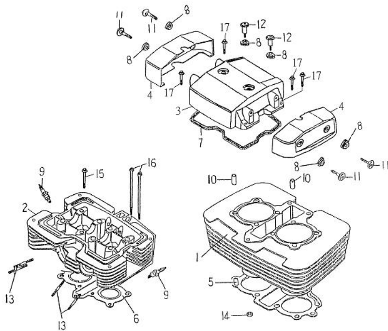
FIG 01 CYLINDER.CYLINDER HEAD
