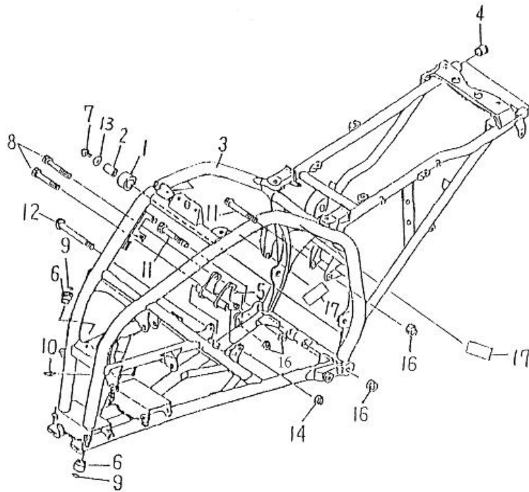
FIG 17 FRAME
