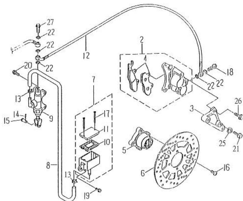
FIG 27 REAR BRAKE
