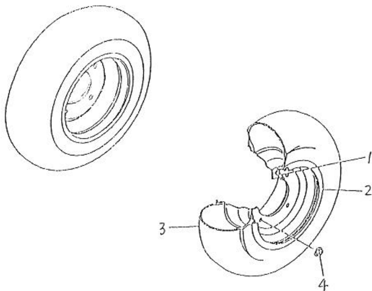
FIG 24 FRONT WHEEL
